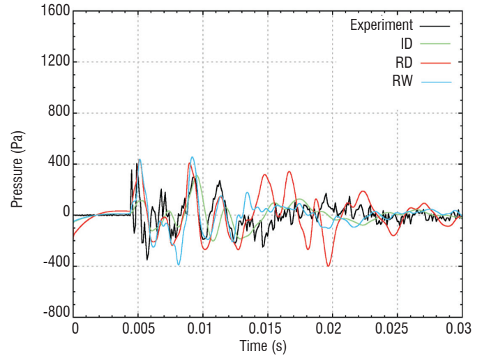
Figure 26 - Experiment/computation comparison ( 120^\circ , 1.5 m)
