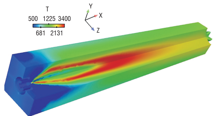
Figure 61 - Temperature field
