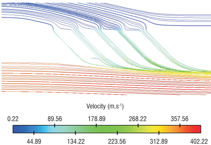
Figure 6 - Velocity streamlines
