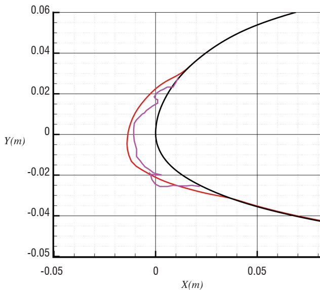
Figure 43 - iced profile normal to the leading edge
