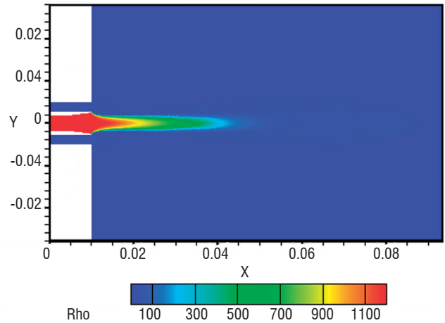
Figure 65 - Density field
