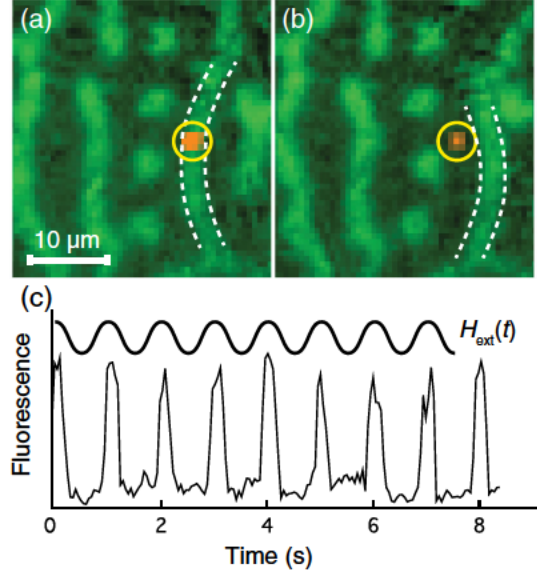
FIG. 3 (color online). Single molecule imaging with simultaneous MO imaging of normal phase domains in the indium film. H_{\text{ext}} is modulated at 1 Hz with a modulation amplitude of 2 Oe around 30 Oe. T = 2.6 \text{ K} . The laser frequency is fixed to the flank of the Lorentzian shaped molecular line. (a) H_{\text{ext}} = 29 \text{ Oe} . A single molecule (the circled bright spot) is chosen above a normal phase domain (delimited by the dashed lines). (b) Image of the same area at H_{\text{ext}} = 31 \text{ Oe} illustrating the motion of the domain boundaries. (c) Temporal evolution of the fluorescence intensity of that molecule probing the flexomagnetolectric effect.
