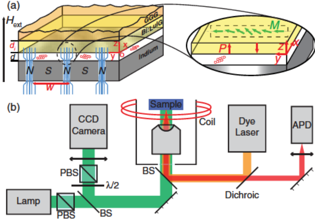
FIG. 1 (color online). Scheme of the sample under an external magnetic field. A hexadecane layer doped with dibenzanthranthrene molecules is squeezed between an indium film and a Bi:LuIG layer grown on a GGG substrate. (Inset) Scheme of magnetization distribution in the Bi:LuIG layer close to a normal phase domain of indium. Electric polarization vectors near the neighboring domain walls have opposite directions. (b) Scheme of the optical setup for single molecule microscopy and simultaneous MO imaging of the regions where the vertical component of the magnetic field penetrates the Bi:LuIG layer.
