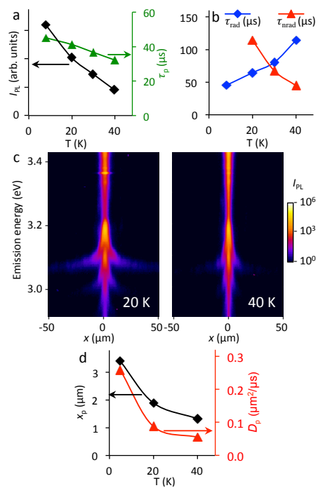
FIG. 4: Temperature dependence in the polar structure of (a) measured spatially and spectrally integrated emission intensity I (black diamonds) and initial decay time \tau_p (green triangles), (b) derived radiative \tau_{\text{rad}} (blue diamonds) and non-radiative \tau_{\text{nrad}} (red triangles) decay times, (c) measured x -energy emission image for IXs, and (d) measured IX transport length x_p (black diamonds) and estimated IX diffusion coefficient D_p = x_p^2 / \tau_p (red triangles). P_{\text{ex}} = 2.4 \mu\text{W} .
