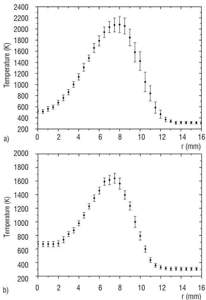
Figure 21 - CARS profiles of temperature measured on N_2 molecules in the two flames; (a): H_2 /air and (b): CH_4 /air.
