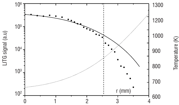
Figure 24 - \text{NO}_2 radial profile obtained by LITG in the \text{CH}_4/\text{air} flame; the signal is decreasing toward the flame, located at r=8\text{mm} , because temperature is increasing and then because of \text{NO}_2 destruction beyond 3 m; measurements (••••), calculation (—) [18] and temperature (dotted). Dashed vertical line indicates the nozzle radius.
