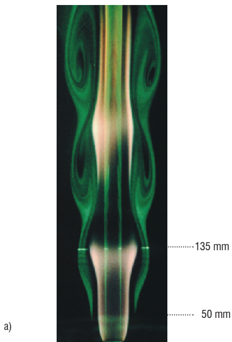
Figure 6 - Buoyant H 2 /air flame, producing vortices at a period of 15Hz, (a): flame; (b):scheme.
