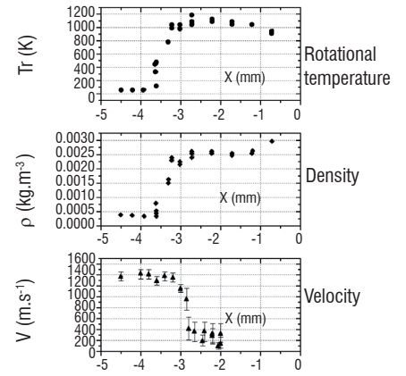
Figure 26 - CARS measurements through a bow shock ; Electron beam fluorescence (EBF) visualization of the shock (left) ; CARS measurements along the stagnation line (right).
