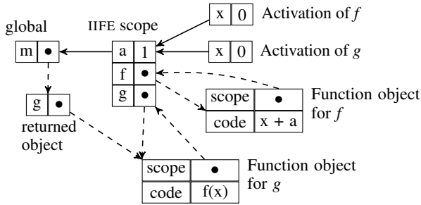
Figure 2. Scope diagram for the call m.g(0) , line 8 of listing 1.
