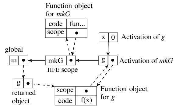
Figure 3. Scope diagram for listing 2.
