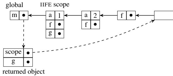
Figure 6. Two scopes are added in front of the IIFE scope. Most references are omitted for legibility.
