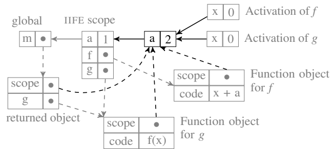
Figure 5. A front scope (highlighted) is added to the module scope. Impacted arrows are highlighted.
