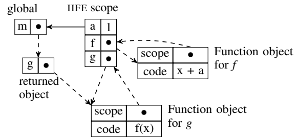
Figure 1. Scope diagram after executing the IIFE of listing 1.
