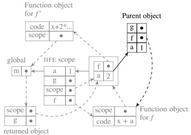
Figure 8. Diagram for listing 7 after line 17. The function object of g is omitted for legibility.
