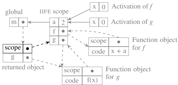
Figure 4. Scope diagram for the call m.g(0) on line 10 of listing 3. The new scope property is highlighted.
