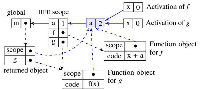
Figure 5. A front scope (in blue) is added to the module scope. Impacted arrows are highlighted in blue.
