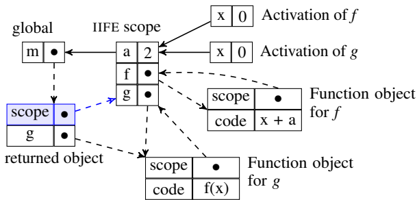
Figure 4. Scope diagram for the call m.g(0) on line 10 of listing 3. The new scope property is highlighted in blue.
