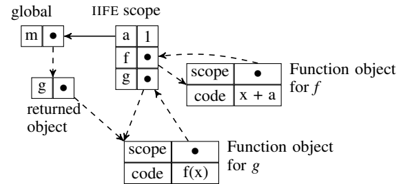
Figure 1. Scope diagram after executing the IIFE of listing 1.
