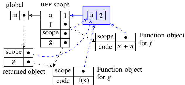
Figure 7. Scope diagram after line 12 of listing 6. The lexical environment created from the with statement and its incoming arrows are in blue.
