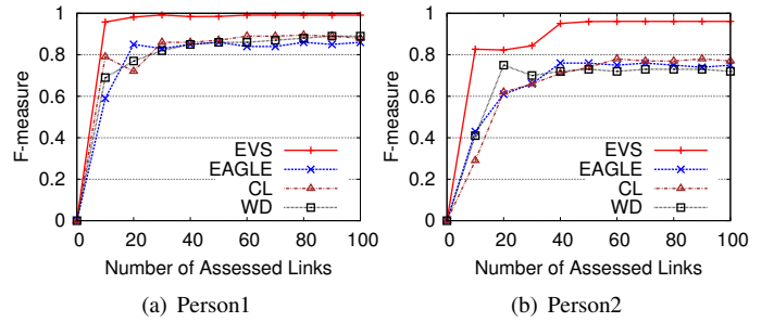
Fig. 1. F-measures of Extended Version Space and Genetic Programming
