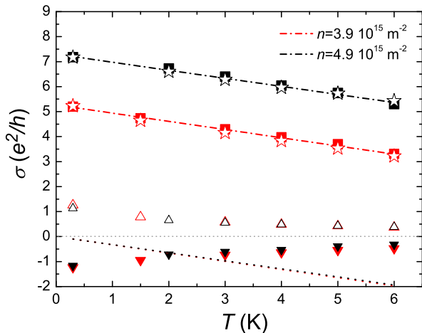
FIG. 2: Temperature dependence of conductivity. Measured conductivity (■), fit of \sigma_D + \sigma_{\text{Ball}} to these data (- · -), Ballistic contribution only (···), diffusive contribution ( \Delta ), WL contribution ( \nabla ) and the sum of Drude, WL, diffusive and ballistic contributions ( \star ). Red symbols correspond to n = 3.9 \times 10^{15} \text{ m}^{-2} and the black symbols to n = 4.9 \times 10^{15} \text{ m}^{-2} . The crossover from diffusive to ballistic regime of interaction is illustrated by the ballistic contribution vanishing at low T while the diffusive one vanishes at high T.
