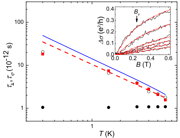
FIG. 3: Phase coherence and intervalley scattering time. Phase coherence (■) and intervalley (●) scattering time obtained by fitting with equations of Ref.32. The black circles (○) are obtained with Hikami formula for B < 0.15 \text{ T} . The dotted red line represents the T^{-1} dependence and the blue solid line represents the prediction of ZNA theory with \mathcal{F}_0^\sigma = -0.67 . The insert shows the experimental magneto-conductivity (black curves) and result of the fit (red curves) for different temperatures ( T = 0.3 \text{ K}, 1.5 \text{ K}, 3 \text{ K}, 4 \text{ K}, 5 \text{ K}, 6 \text{ K} from top to bottom.). The arrow indicates the crossover field B_v \approx 0.25 \text{ T} (See the text).
