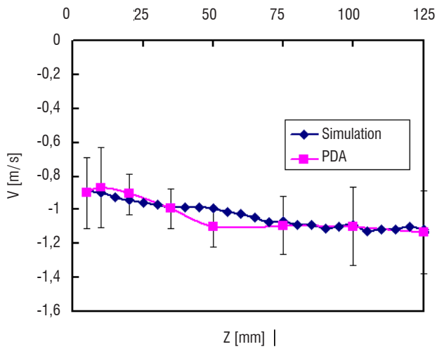
Figure 15 - Longitudinal change in the droplet's velocity ( Y=0 mm)
