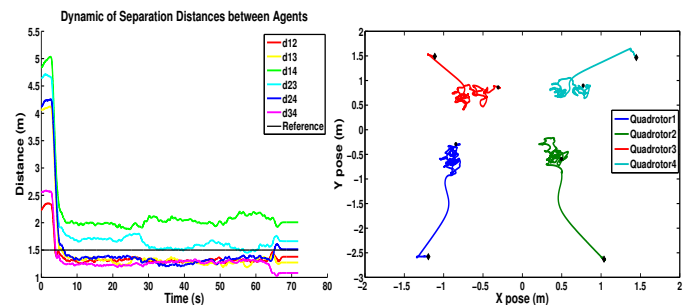
Fig. 3: (Left) Interdistances between 4 quadrotors in the real-time experiment by using the control law in (20). Once the control law of flocking is launched in each quadrotors, the interactions start and the distances converge. Finally, the quadrotors land after t = 60s . (Right) Trajectories of 4 quadrotors in the real-time experiment by using the control law in (20). Quadrotors move from their initial positions to the destination point, gather around the center and form a quasi- \alpha -lattice
