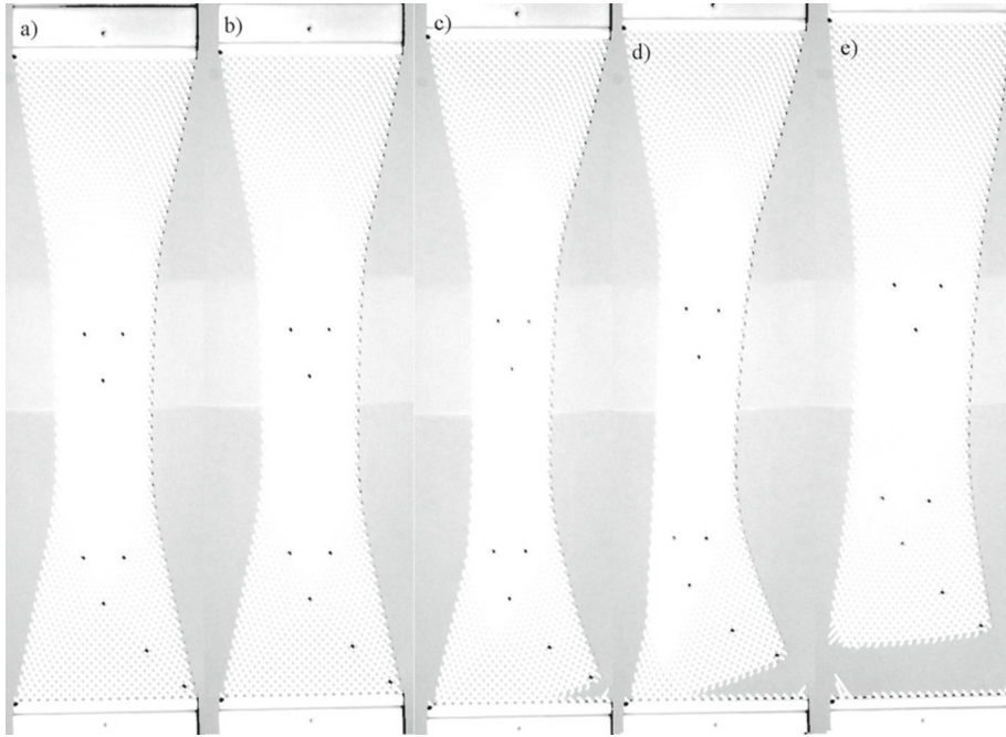
FIG. 17. Tensile test of sample 1 (see also Fig. 20) a) sample under stretch before first beam breakage, b) fiber connected to the lower left-hand side corner deterioration, c), d) damage of further fibers, e) complete deterioration of the sample
