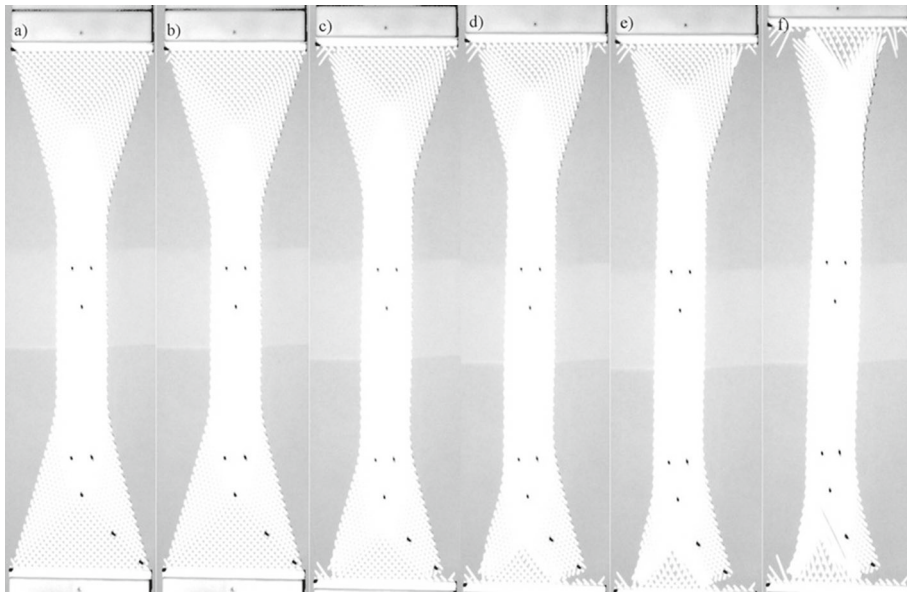
FIG. 18. Tensile test of sample 2 (see also Fig. 21): a sample under stretch before first beam breakage, b fiber connected to the upper left-hand side corner deterioration, c-f damage of further fibers
