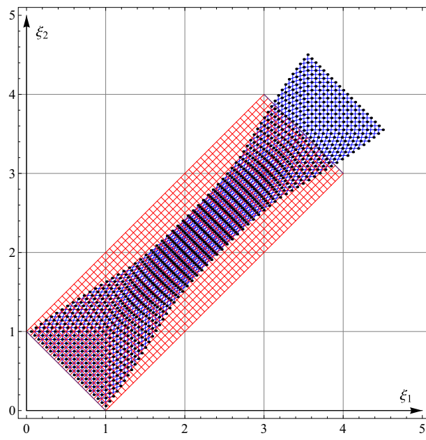
FIG. 9. Deformed configuration for u_x = u_y = 0.6 * L , \alpha = 5 and \beta = 1
