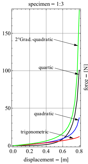
FIG. 12. Force–displacement curve for the considered energy model
