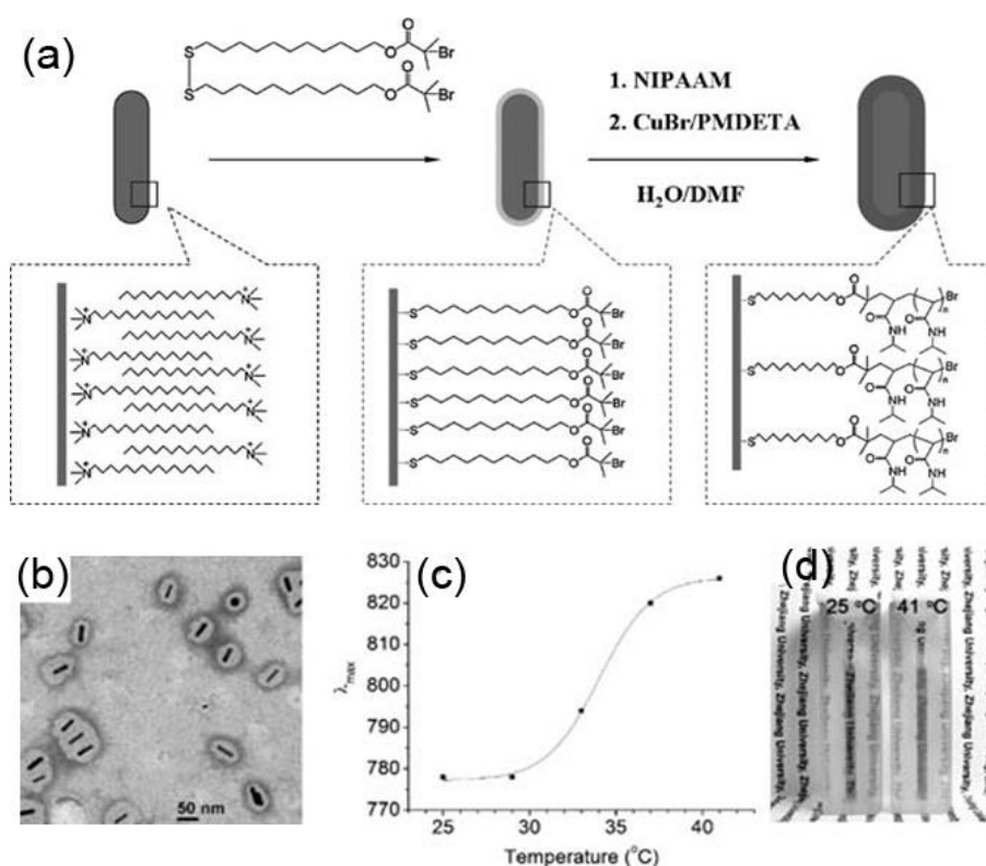
Fig. 3 Preparation of GNR/PNiPAAM hybrid nanostructures via surface-initiated ATRP (a), representative TEM image of GNR/PNiPAAM nanohybrids (b), the fitted plotting of longitudinal surface plasmon wavelengths of GNR/PNiPAAM vs. temperature (c), and digital photographs of GNR/PNiPAAM solutions at 25 and 41°C, respectively. Adapted with permission from Ref. 93. Copyright 2008 WILEY-VCH Verlag GmbH & Co. KGaA, Weinheim.
