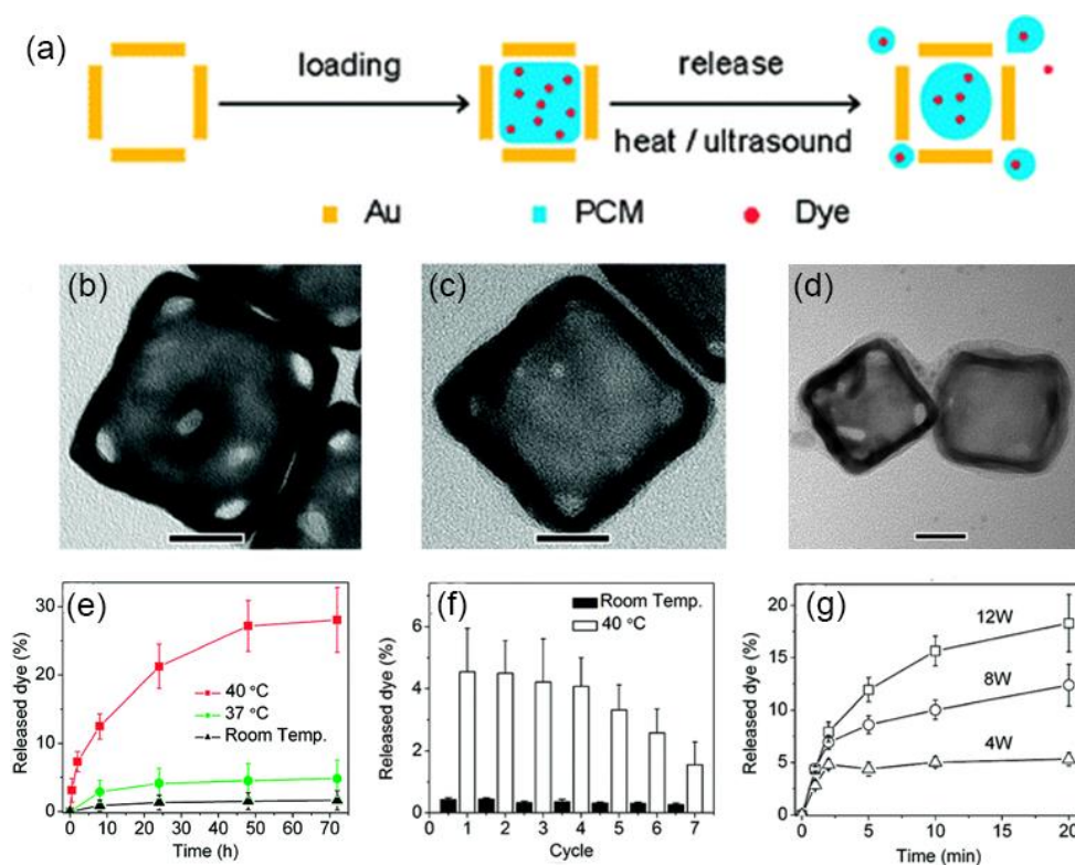
Fig. 12 Schematic illustration on how to load the hollow interior of a gold nanocages with a dye-doped PCM and then have it released from the gold nanocages by direct or ultrasonic heating (a); TEM image of pristine gold nanocages (b), drug loaded nanogels before (c) and after (d) HIFU application. Release profiles of R6G under direct heating to various temperatures for different periods (e); pulsatile release under alternative heating/cooling cycles (f), and release profiles of R6G by HIFU at different applied powers (g); and (c). Adapted with permission from Ref. 198. Copyright 2011 American Chemical Society.
