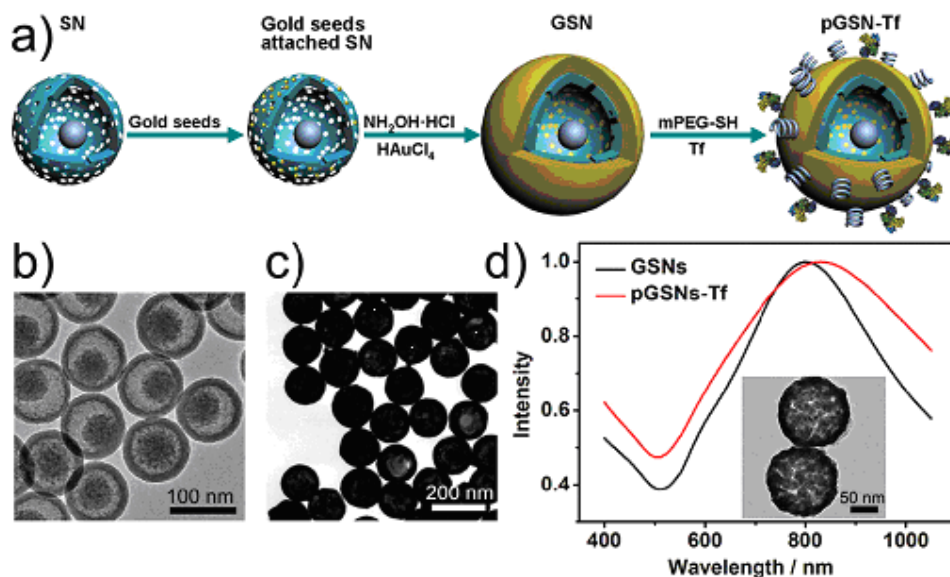
Fig. 10 a) Schematic diagram of gold-coated silica nanorattles (GSNs) synthesis and bio-conjugation; b) TEM image of silica nanorattles (SNs); c) TEM image of GSNs and d) extinction spectra of the GSNs after PEGylation (pGSNs) and marking with targeting ligands of transferrin (pGSNs-Tf), the inset is the TEM image of pGSNs-Tf. Adapted with permission from Ref. 202. Copyright 2012 WILEY-VCH Verlag GmbH & Co. KGaA, Weinheim..
