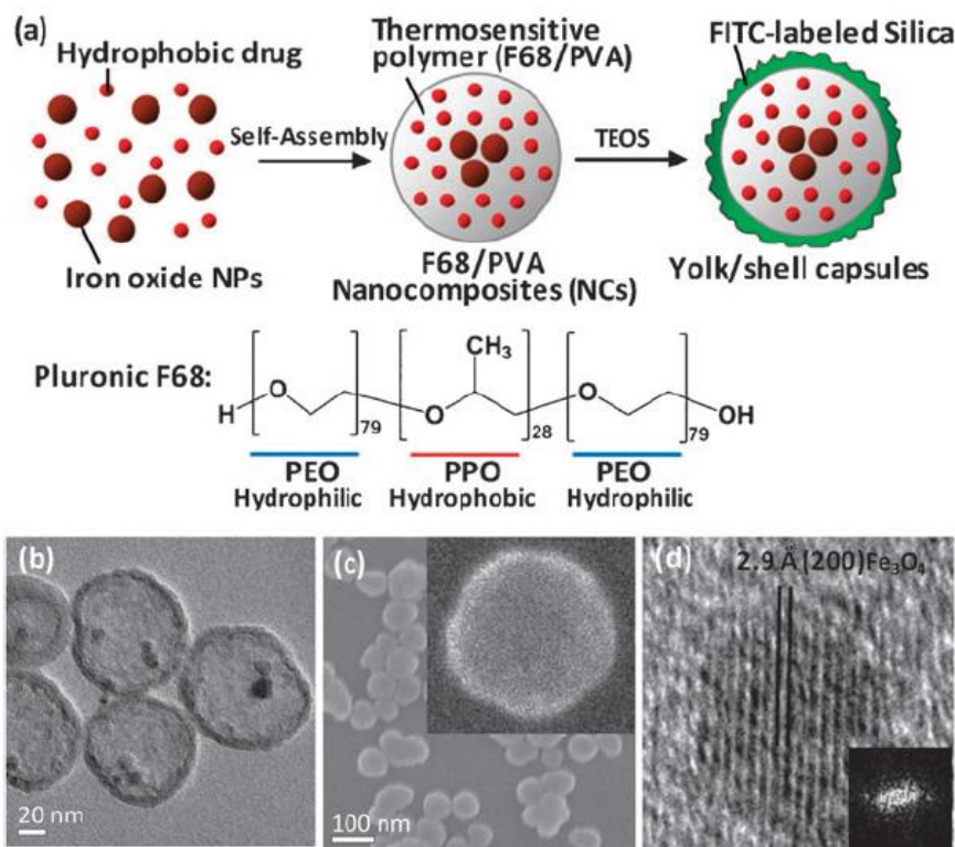
Fig. 9 Schematic illustration of the synthesis and structure of the hollow silica nanostructure for magnetically-triggered controlled drug release. The first step involved mixing the iron oxide nanoparticles and the hydrophobic drug in an organic solvent to form a uniform phase. Next, the mini-emulsion method was applied using blended polymers, poly(vinyl alcohol) (PVA) and Pluronic® F68 (PEO-PPO-PEO) as a binder to fabricate the self-assembling nanocomposites. Upon the evaporation of the organic solvent, the polymers encapsulated the iron oxide nanoparticles and hydrophobic drug within the composite. Finally, the nanocomposites were coated with a thin layer of silica by hydrolysis and condensation of TEOS to obtain the final yolk/shell capsules (a). This nanostructure possesses an average diameter of about 76 nm and 7-nm ultra-thin silica shell (b, c and d). Adapted from Ref. 192 with permission from The Royal Society of Chemistry.
