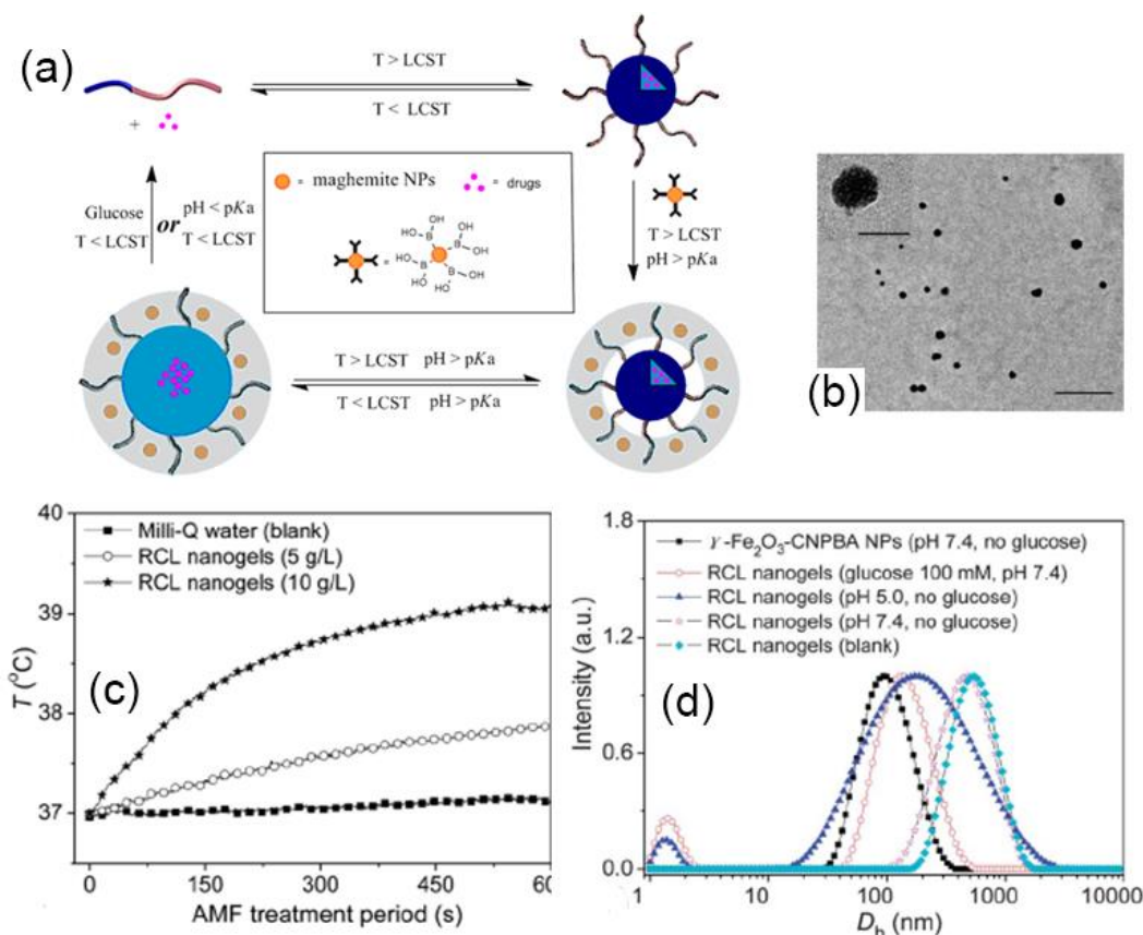
Fig. 5 Preparation of reversibly cross-linking (RCL) nanogels from PVOH- b -PNVCL with surface-functionalized \gamma -Fe 2 O 3 NPs via the boronate/diols bonding and loading of hydrophobic cargoes (a); representative TEM image of the RCL nanogels (scale bar: 500 nm), and inset: partially-magnified TEM image of a nanogel particle (scale bar: 100 nm) (b); AFM-induced heating profiles of the RCL nanogel aqueous solutions (10 and 5 g L -1 ) under
