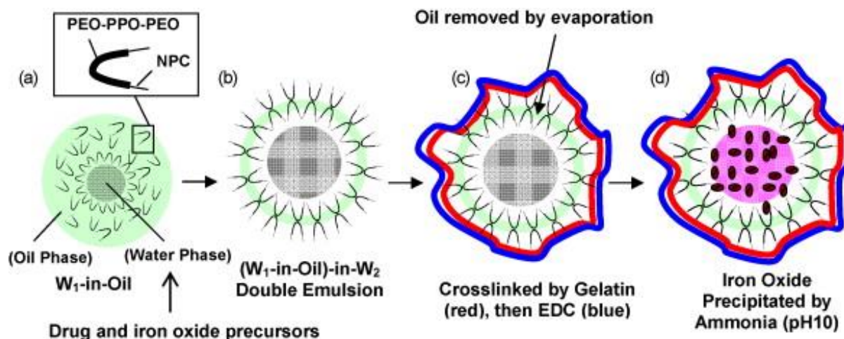
Fig. 6 A self-assembly strategy of aqueous nanovehicles using double emulsion for drug delivery under combined magnetic and thermal stimuli. “W 1 ”: a water phase made of PBS/hydrophilic drug/Fe salts mixture, “W 2 ”: PBS buffer, “Oil”: PEO-PPO-PEO/CH 2 Cl 2 solution. The PEO-PPO-PEO was end-functionalized with 4-nitrophenylchloroformate (NPC) for subsequent cross-linking with gelatin. (a) Adding W 1 to oil phase to form an inverse micelle emulsion; (b) adding this emulsion to W 2 to form micelle dispersion with a PEO-PPO-PEO shell; (c) the PEO shell was cross-linked with gelatin at 4 °C with 1-ethyl-3-(3-dimethylaminopropyl)- carbodiimide (EDC) as catalyst; meanwhile, CH 2 Cl 2 residue can be removed by evaporation; (d) iron oxide nanoparticles can be precipitated by adding ammonia to raise pH to 10 under modest heating of 60 °C. Adapted from Ref. 14, copyright 2009 Elsevier.
