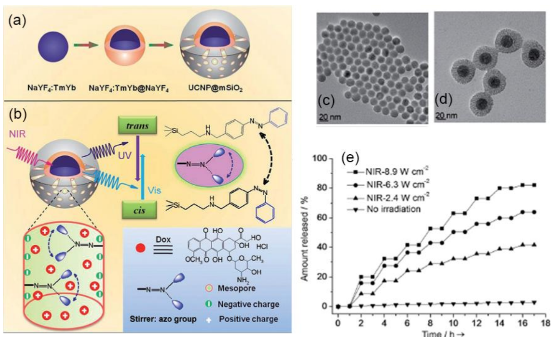
Fig. 15 a) Synthetic procedure for upconverting nanoparticles coated with a mesoporous silica outer layer (a), NIR light-triggered DOX release by making use of the upconversion property of UCNPs and trans-cis photoisomerization of azobenzene moieties introduced in the mesopore network of a mesoporous silica layer (b). TEM images of NaYF 4 :Tm,Yb (c) and NaYF 4 :Tm,Yb@NaYF 4 @mSiO 2 (d); drug release in PBS under NIR light irradiation (980 nm, 8.9 W cm -2 , 1s) and dark conditions, alternatively (e). Adapted with permission from Ref. 232. Copyright 2013 WILEY-VCH Verlag GmbH & Co. KGaA, Weinheim.
