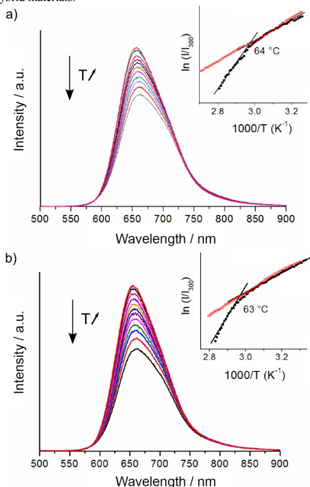
Figure 2. Temperature dependent emission spectra ( \lambda_{exc}=400 nm) of Kat 2 [Mo 6 I 8 (C n F 2n+1 COO) 6 ] a) n = 2, b) n = 3. Inset : evolution of signal intensity at 656 nm in function of temperature for the hybrid (in black) and their respective cesium precursor (in red)
