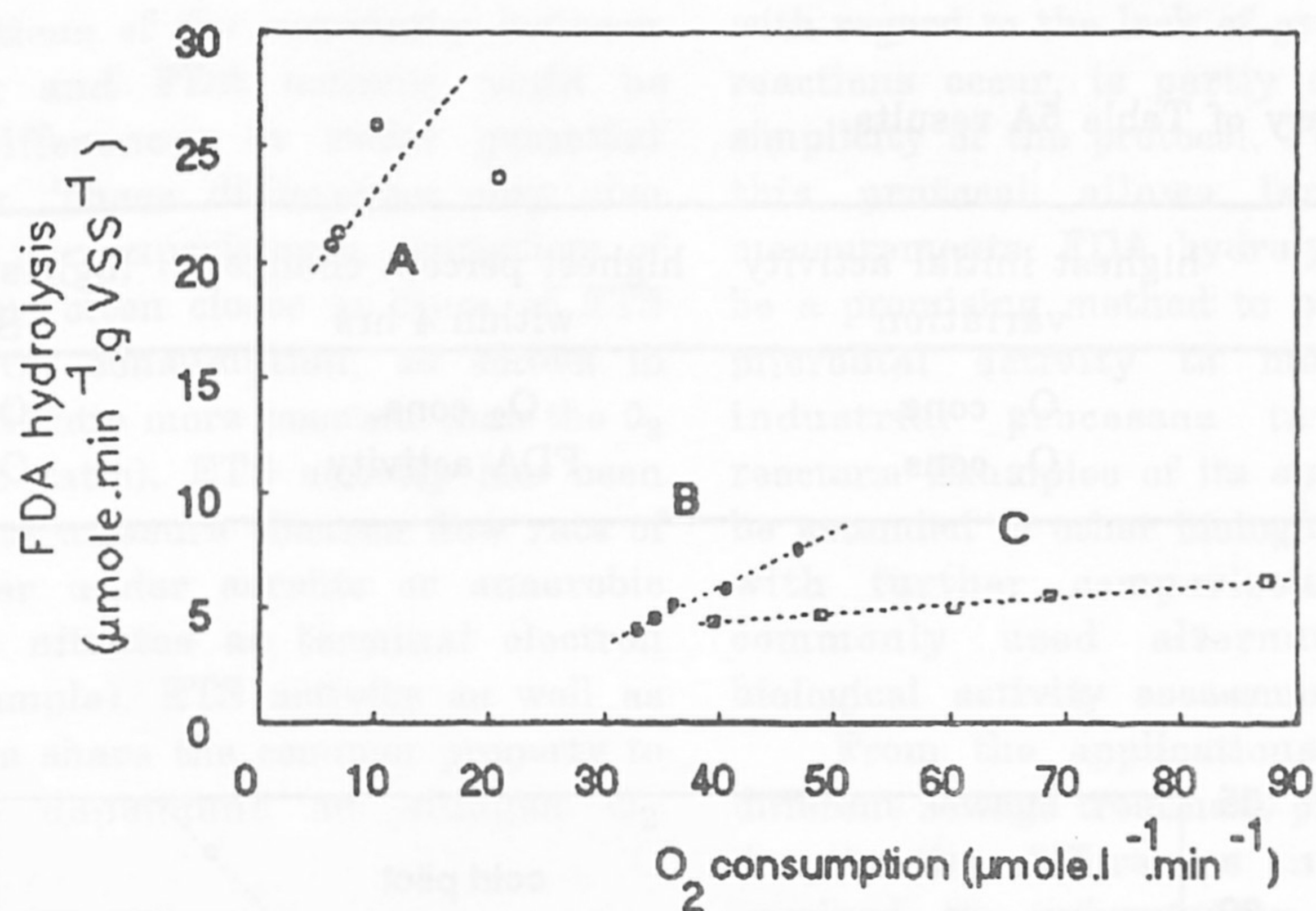
Figure 5. Relationships between FDA hydrolysis and O_2 consumption. A : sludge sample from a pilot treatment plant during endogenic respiration. B : sludge sample from Fontenay Tresigny sewage treatment plant. C : sludge sample from a pilot treatment plant with regular trophic supply.
