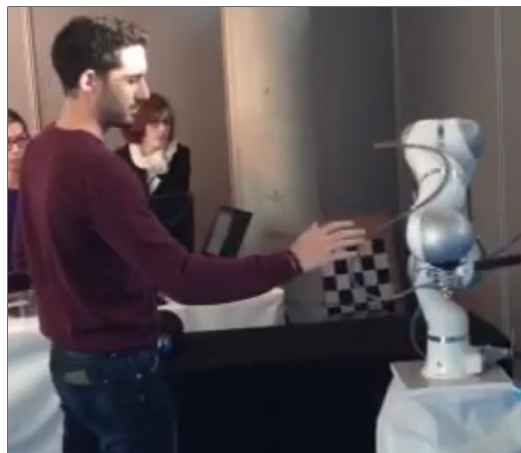
Fig. 1. View of a user sharing its workspace with the KUKA LWR manipulator. The kinetic energy of the system is modulated as a function of the distance between the human operator and the end-effector of the robot in order to best perform the task of the robot while ensuring safety.
