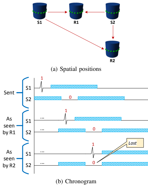
Fig. 1. "0" symbols can be masked by "1" even if not sent at the same time
