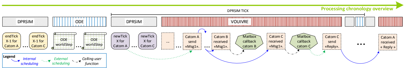
Fig. 8: Global processing overview and mailbox callbacks
