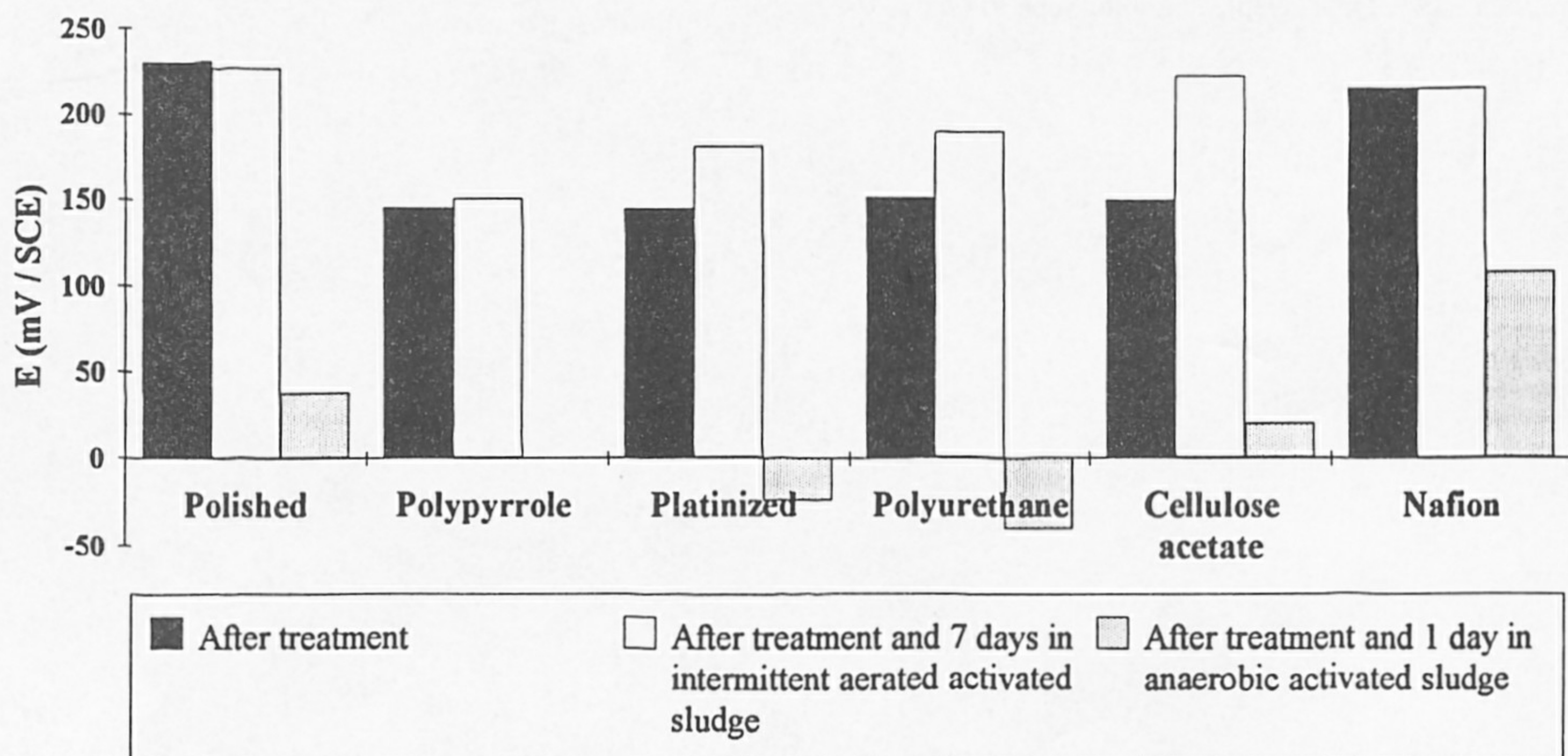
Fig. 2. Zero-current potentials in treated water or aerated activated sludge.
