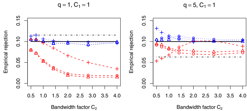
FIG 2. Empirical rejections under H_0 as a function of the bandwidth, n = 100 .
