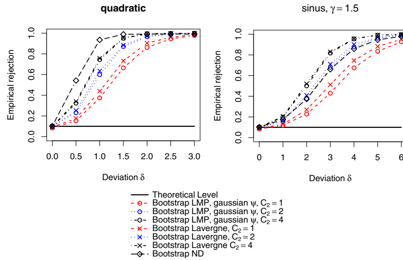
FIG 7. Empirical power curves, X Bernoulli and n = 100 .
