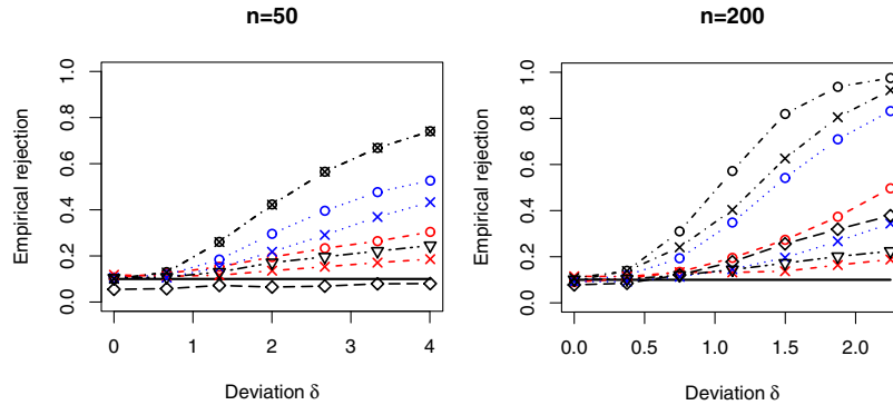
FIG 4. Empirical power curves for a quadratic alternative, q = 5 .
