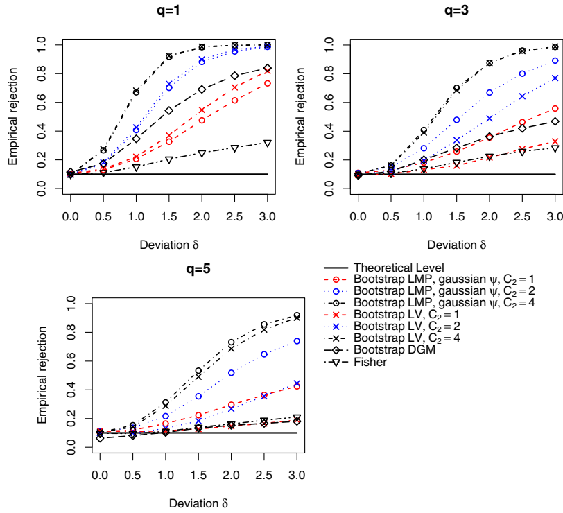
FIG 3. Empirical power curves for a quadratic alternative, n = 100 .
