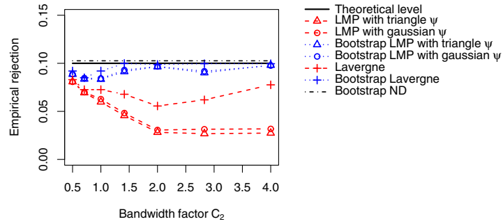
FIG 6. Empirical rejection under H_0 as a function of the bandwidth, X Bernoulli and n = 100 .
