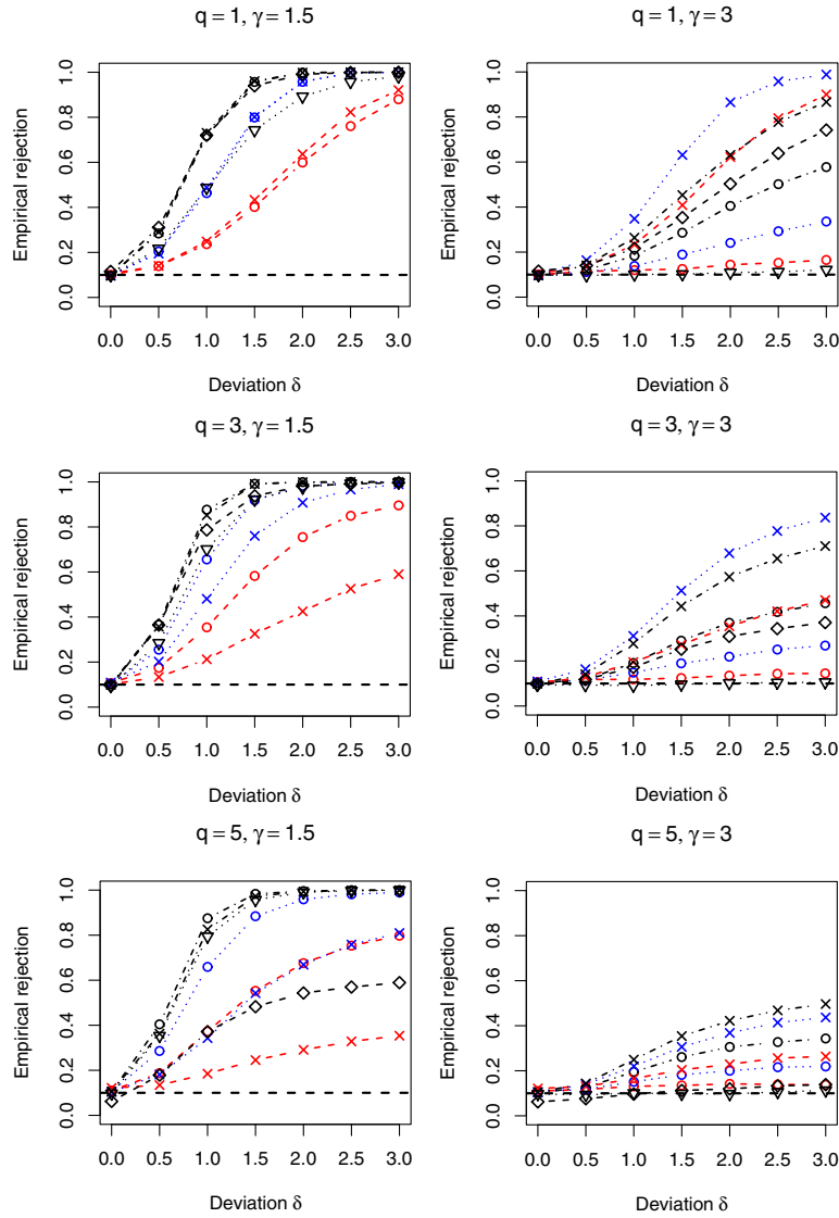
FIG 5. Empirical power curves for sine alternative, n = 100 .
