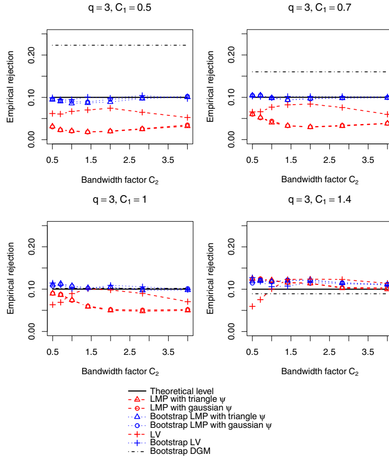
FIG 1. Empirical rejections under H_0 as a function of the bandwidth, n = 100 .
