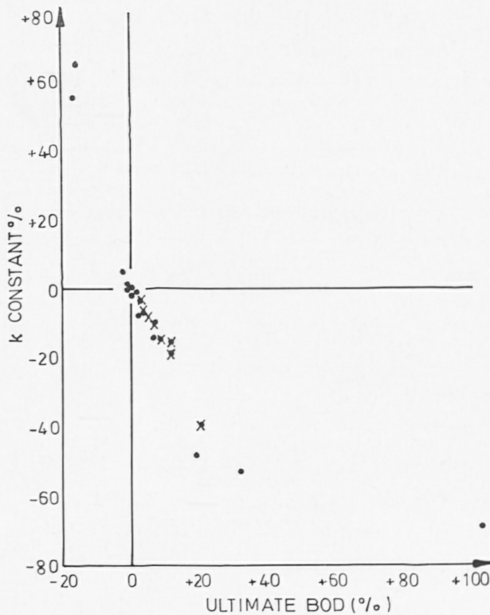
Fig. 12.3: Biodegradation kinetic constant determination: deviation from the best estimate. After Marske et al., 1972. o: Method of Moments, x: Thomas Slope Method, •: Log-difference Method.
