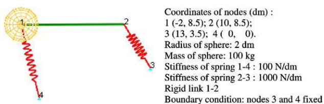
Fig. 6. Free drop of system 'mass-spring-rigid link'.
