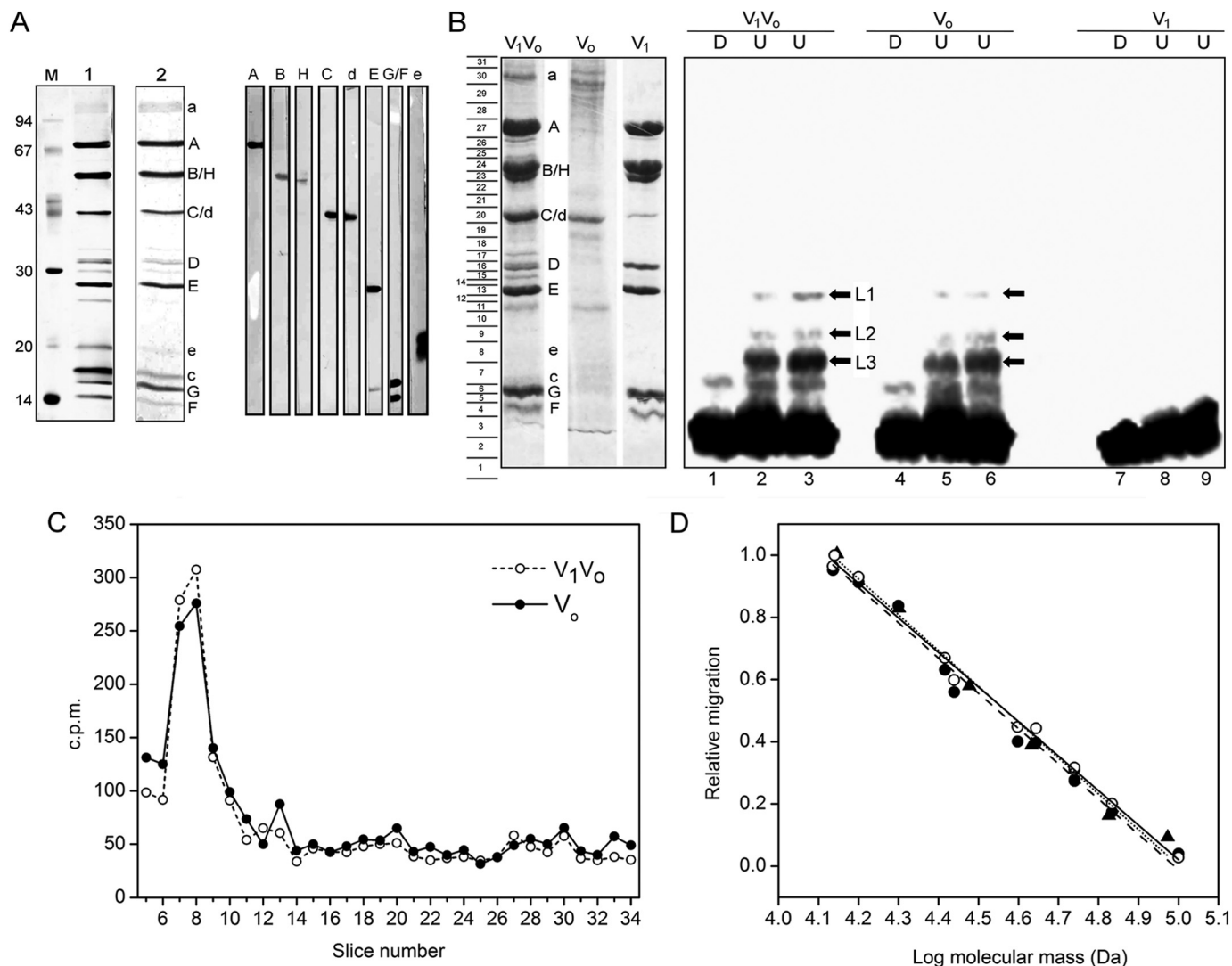
FIGURE 4. Characterization of PA1b binding. A, left , SDS-PAGE analysis of purified M. sexta V-ATPase with staining with silver ( lane 1 ) or Coomassie Brilliant Blue ( lane 2 ) and M indicating molecular mass markers. Right , identification of the staining polypeptides by immunoblot analysis. B , photoaffinity labeling of M. sexta V-ATPase with the ^{125}\text{I} -PA1b-benzophenone. For labeling, V_1V_0 holoenzyme ( V_1V_0 ), V_0 complex ( V_0 ), or V_1 complex ( V_1 ) was incubated with ^{125}\text{I} -PA1b-benzophenone and exposed to UV light or kept in the dark. After separation by SDS-PAGE, the stained and dried gel was exposed to a phosphorimaging screen. Left , SDS-PAGE of the V-ATPase complexes with Coomassie Blue staining. Right , readout of the phosphorimaging screen for labeled holoenzyme ( lanes 1–3 ), V_0 ( lanes 4–6 ), and V_1 ( lanes 7–9 ) after either UV irradiation (U) or maintenance in the dark (D). Bands L1–L3 ( arrows ) indicate UV-dependent labeled species. C , slices of the dried gel from samples of the V_1V_0 holoenzyme ( open circles ) and V_0 ( filled circles ) subjected to scintillation counting. The column to the left of B indicates positions of gel slices subjected to counting. The majority of the radioactivity was found in slice 3 near the dye front. D , molecular mass determination of ^{125}\text{I} -labeled V-ATPase subunits. A calibration curve was prepared by plotting log molecular masses of standard proteins ( triangles, dashed line ) and V-ATPase subunits (deduced from their primary structure) against their relative migration on the SDS-polyacrylamide gels shown in A ( open circles, dotted line ) and B ( filled circles, solid line ). In each case, linear regression gave r^2 > 0.99 .
