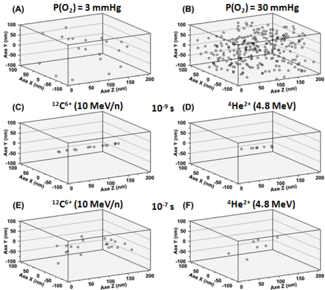
Figure 4. Spatial distributions of oxygen molecules dissolved in water at a partial pressure of 3 mmHg (A) and 30 mmHg (B) or produced in the track of C[10 MeV/n] (LET=168 keV/ \mu\text{m} ) and He[1.2 MeV/n] (LET=94 keV/ \mu\text{m} ) at 10^{-9} s C and D) and 10^{-7} s (E and F) after ion impact [29]. 3 mmHg and 30 mmHg correspond to the range of partial pressures at which OER begins to saturate for various cell lines.
