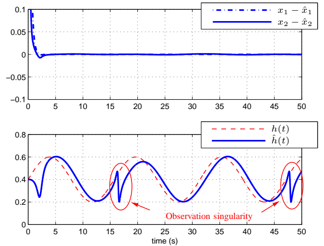
Fig. 6. Simulation 4 with h(t) = h_2(t) and u(t) = u_2(t) (sine)
