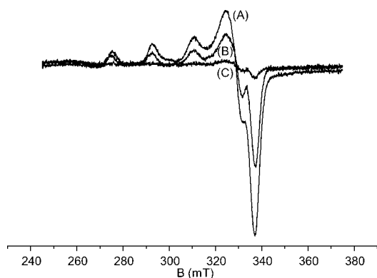
Figure 1. Evolution of the X-band EPR spectra of [\text{Ru}^{\text{II}}_{\text{phot}}\text{-Cu}^{\text{II}}_{\text{cat}}] ( 10^{-4} M + 200 molar equiv TEOA) in \text{CH}_3\text{CN} , under argon after irradiation at 450 nm. A) t=0 , B) t=1 min, and C) t=5 min at 100 K.
