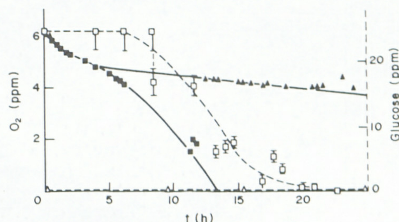
Fig. 3. DO (—) and glucose (---) concentration changes in Seine water samples either crude ( \blacktriangle \triangle ) or added with 25 \text{ mg l}^{-1} glucose ( \blacksquare \square ) and incubated at 20^\circ\text{C} .
