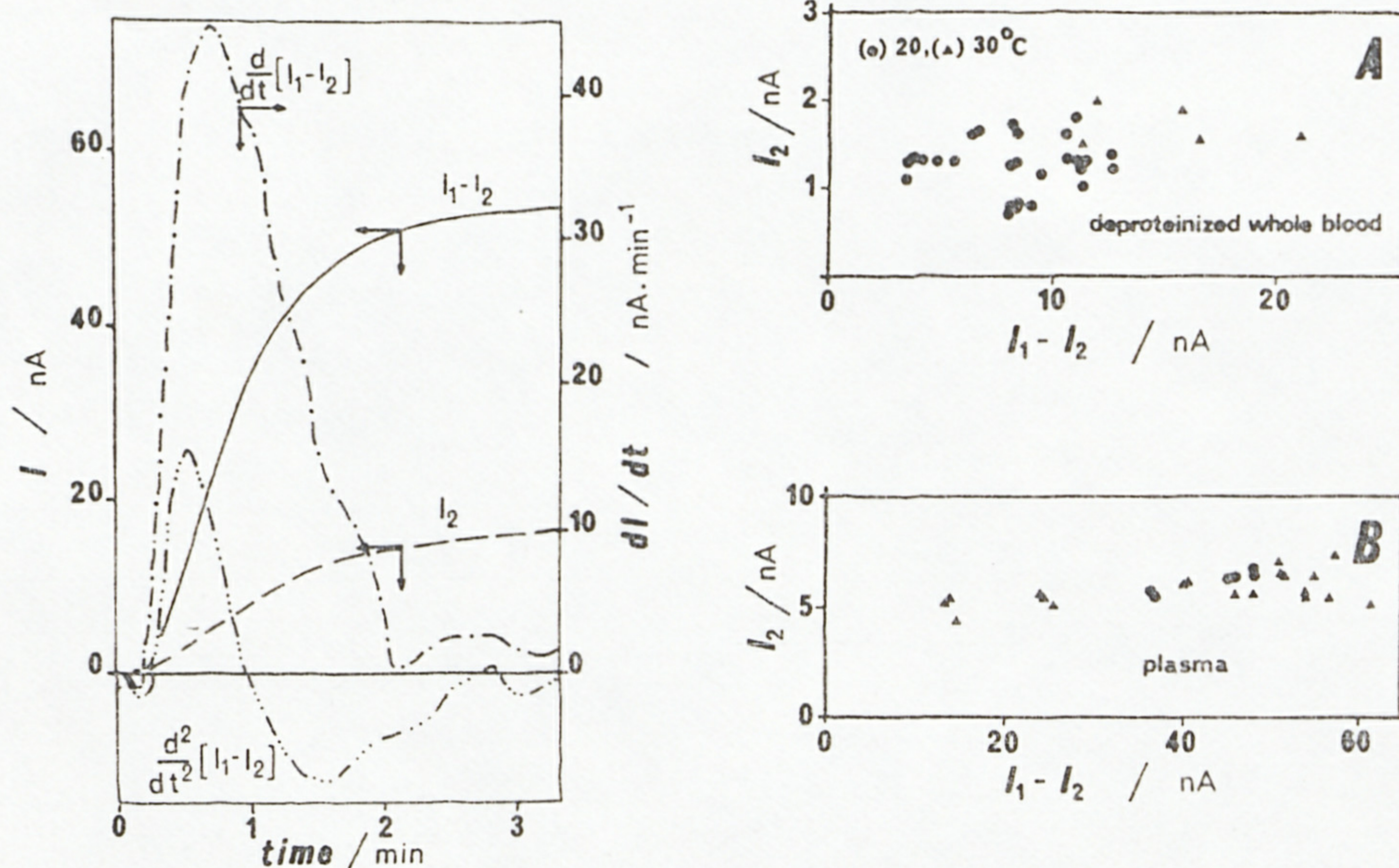
Figure 1 - Response curves for a 50 \mu l blood plasma sample.
