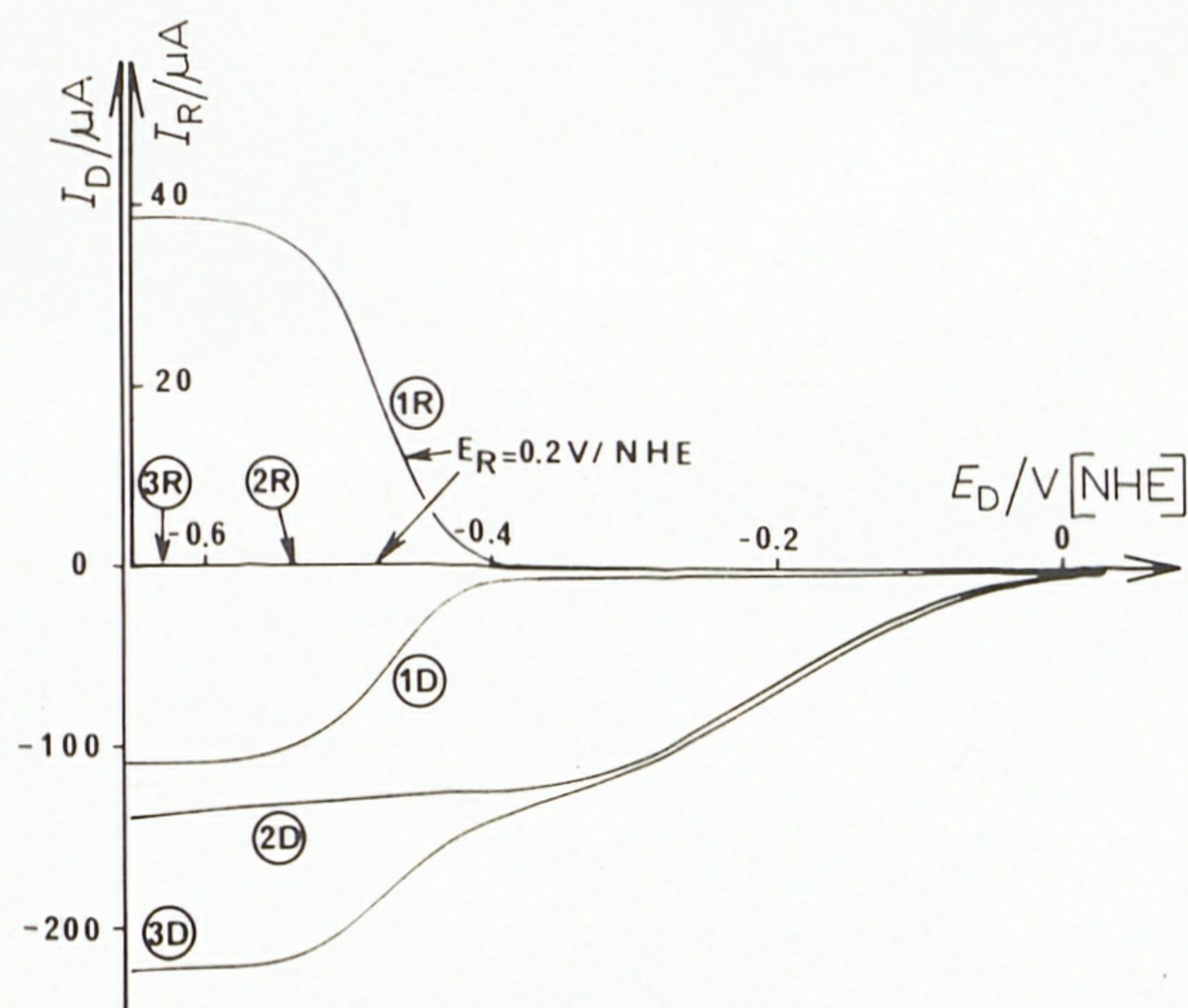
Fig. 4. Reactivity of MV^{2+} towards dissolved oxygen. Phosphate buffer (pH 6.8), electrode No. 1, monitored ring-disc potential +0.2 V/NHE. Concentration of methyl viologen: (1) and (3) 1 mM, (2) 0 mM. Concentration of oxygen: (1) 0 mM, (2) and (3) 0.29 mM, i.e., air saturated at 20°C.
