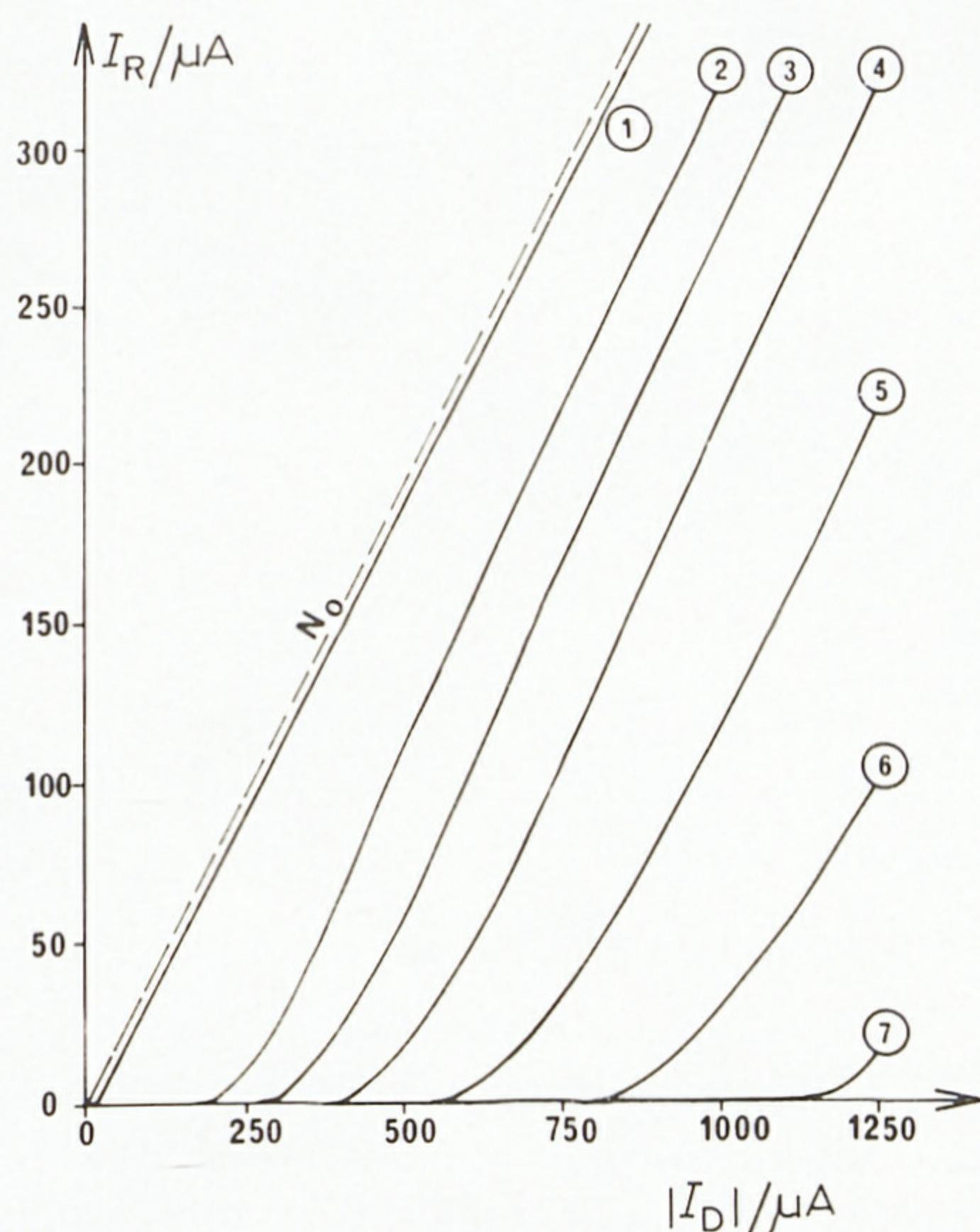
Fig. 5. Oxygen titration curves by electrogenerated MV^{*+} : ring current versus disc current curves at different oxygen concentrations. Phosphate buffer (pH 6.8), electrode No. 1, monitored ring potential +0.2 V/NHE. MV^{2+} 10 mM, concentration of oxygen (1) 0, (2) 0.20, (3) 0.35, (4) 0.46, (5) 0.72, (6) 1.0, (7) 1.45 mM; (---) line of slope N_0 (Table 1).
