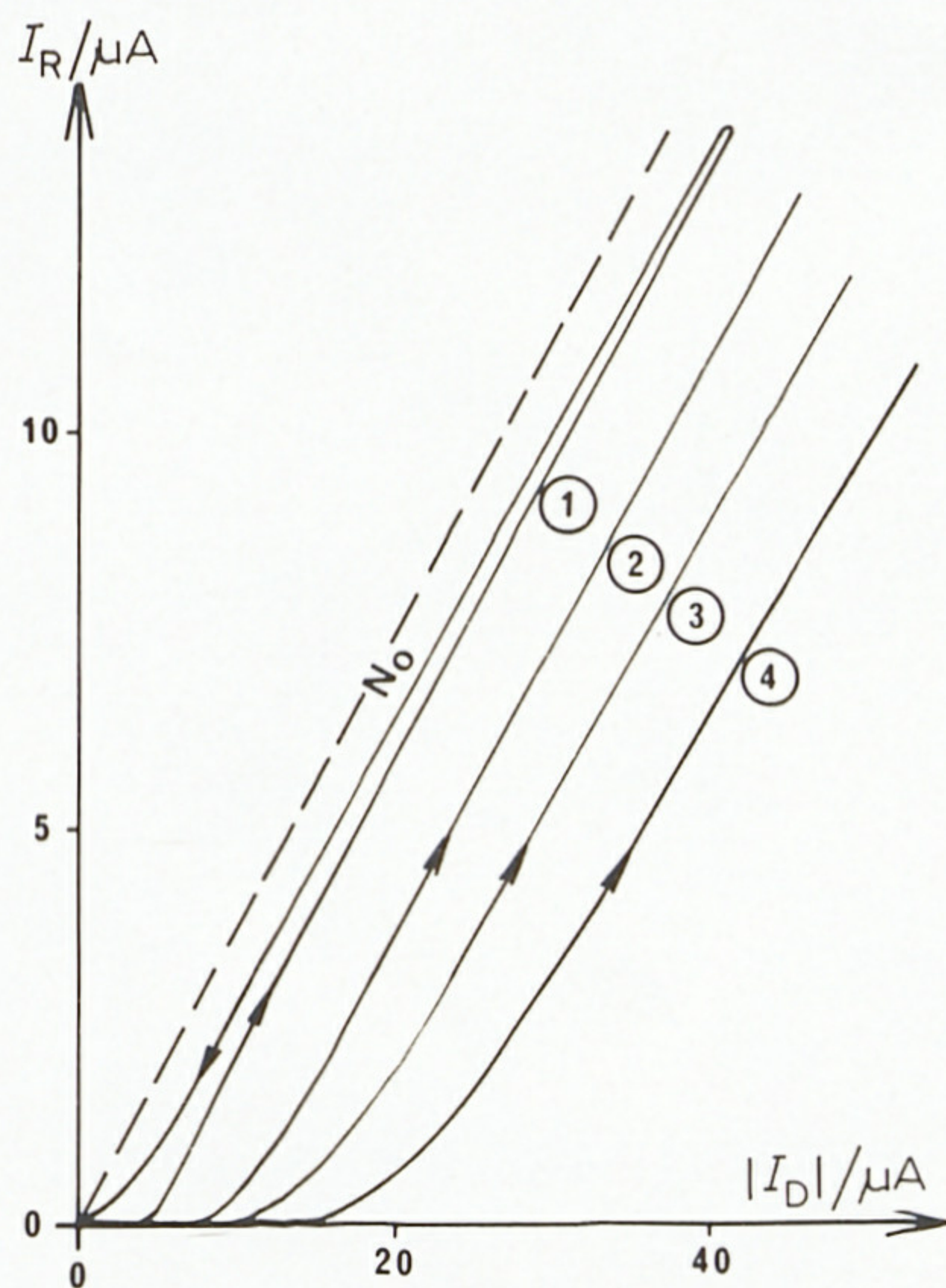
Fig. 7. Horse heart cytochrome c titration curves by electrogenerated BV^{•+} ring current versus disc current curves at different cytochrome c concentrations. Phosphate buffer (pH 6.8), electrode No. 1, monitored ring potential +0.1 V/NHE, BV^{2+} 1.24 mM. Cytochrome c (1) 0, (2) 40, (3) 80, (4) 120 \mu M ; (---) line of slope N_0 (Table 1).
