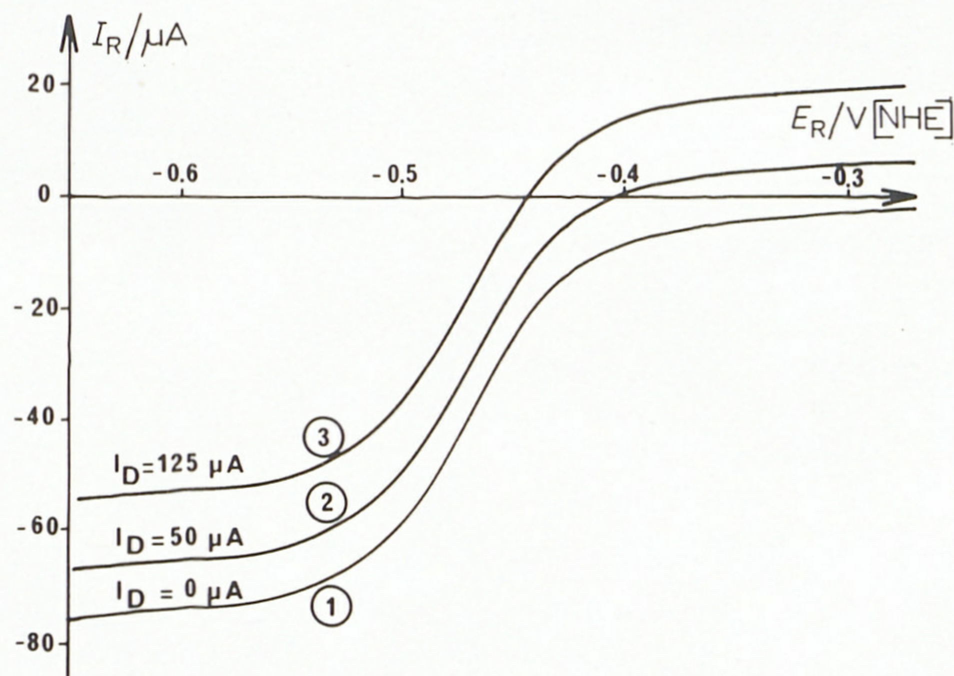
Fig. 1. Reversibility of MV^{2+}/MV^{•+} : influence of the monitored disc current on the ring voltammetric curves in a 1.1 mM MV^{2+} solution. Phosphate buffer (pH 6.8), electrode No. 1. Monitored disc current value: (1) 0 \mu A , (2) 50 \mu A , (3) 125 \mu A . Limiting value of the disc current for the first MV^{2+} reduction wave: 115 \pm 5 \mu A .
