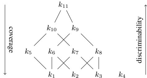
Figure 1. The set of candidate linkkeys. This is a subset of the powerset lattice \langle 2^P \times P', \subseteq \rangle , but not a lattice.
