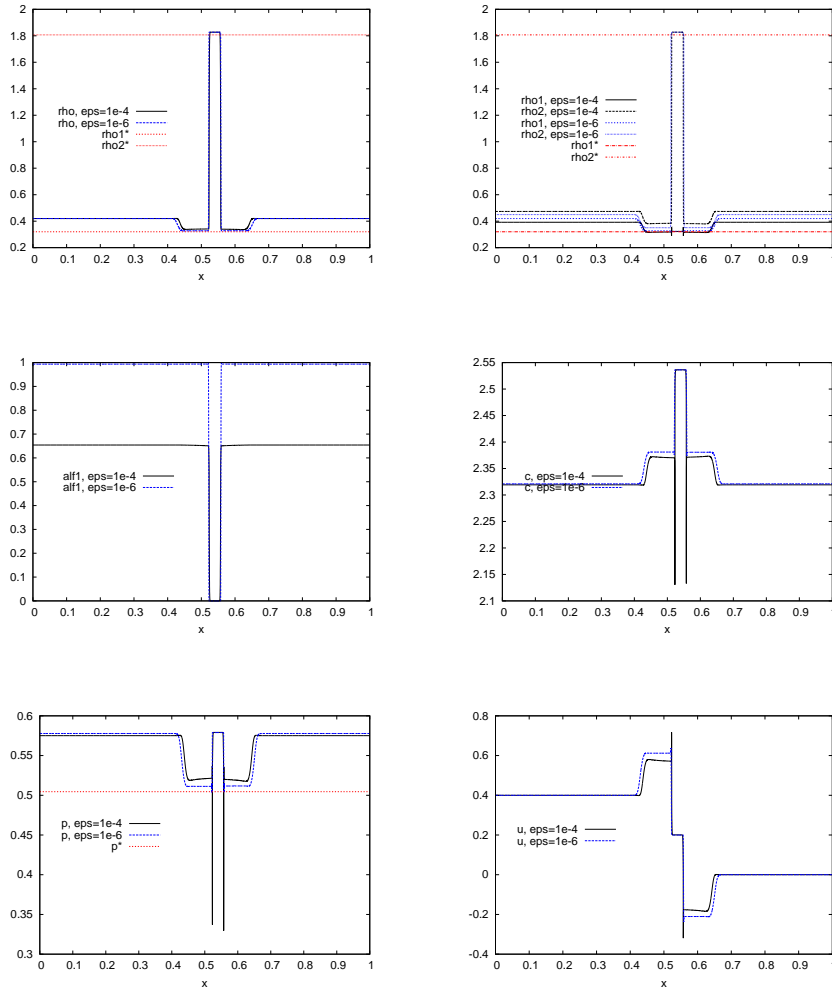
FIGURE 14. Perturbation of a metastable state at t=0.2s . From top left to bottom right: density \rho , densities \rho_{\alpha_1} and \rho_{\alpha_2} , volume fraction \alpha_1 , speed of sound c , pressure p and velocity u .
