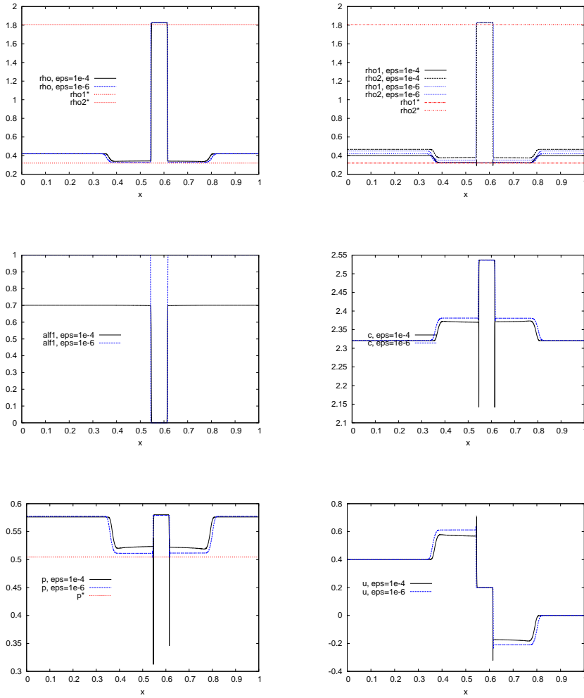
FIGURE 15. Perturbation of a metastable state at t=0.4s . From top left to bottom right: density \rho , densities \rho_{\alpha_1} and \rho_{\alpha_2} , volume fraction \alpha_1 , speed of sound c , pressure p and velocity u .
