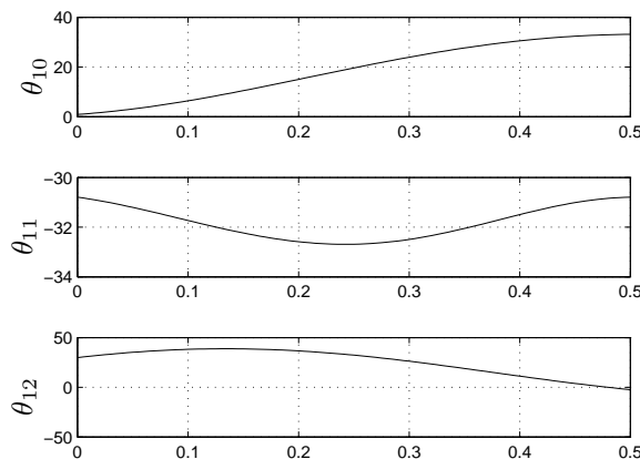
Fig. 8. Joints variables \theta_{10} , \theta_{11} , and \theta_{12} (°) as a function of time (s), respectively for the upper leg, the lower leg and the shoe, connected with the swing leg of the biped.
