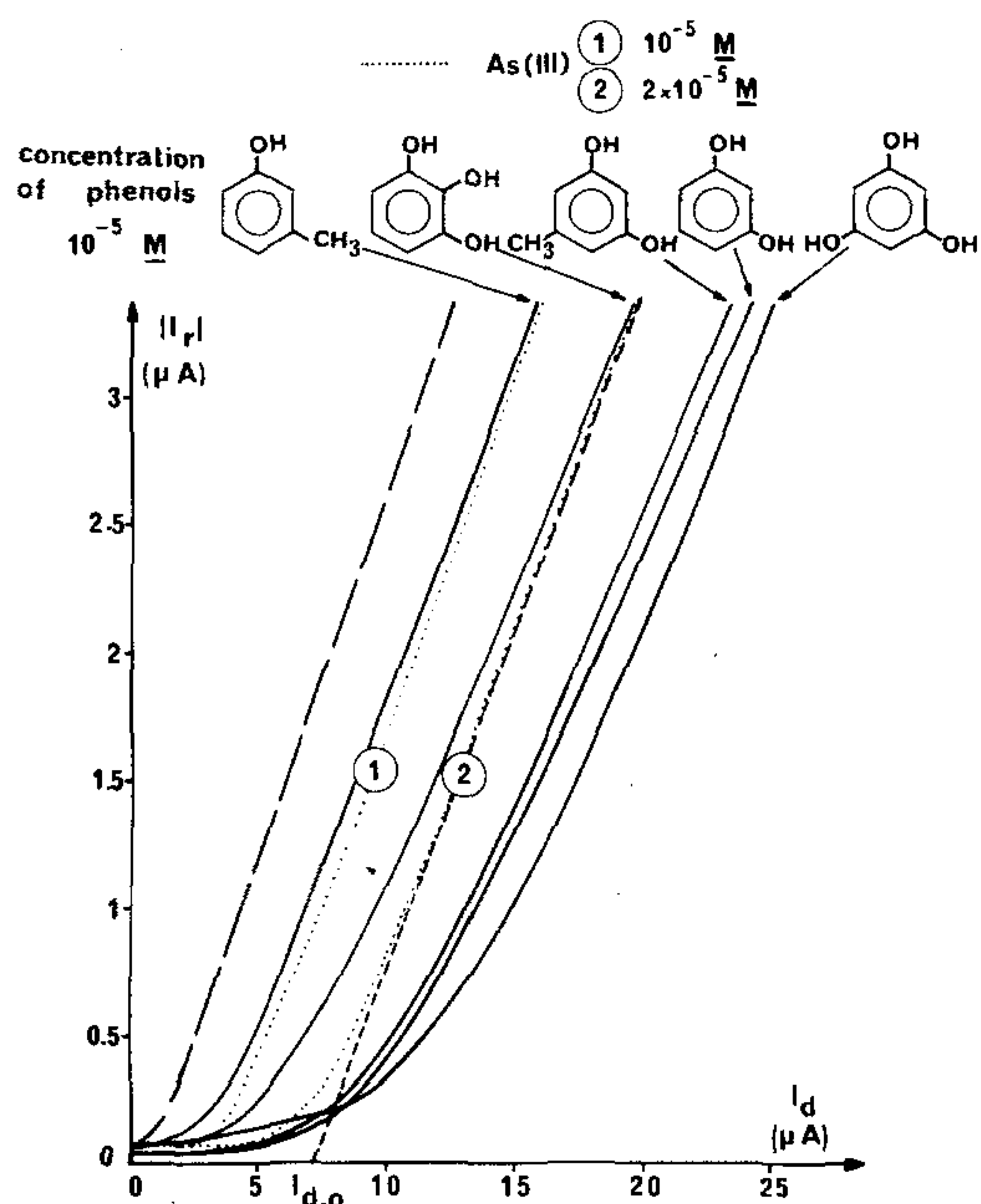
Fig. 1. Titration curves of 10^{-5} M solutions of m.cresol, pyrogallol, orcinol, resorcinol and phloroglucinol; comparison curves (.....) with 10^{-5} M (1) and 2 \times 10^{-5} M (2) As (III) solutions. Gold ring-carbon disc electrode (No. 1), \text{H}_2\text{SO}_4 1 N, \text{Br}^- 0.5 M, W = 28.6 Hz, 25^\circ\text{C} .
