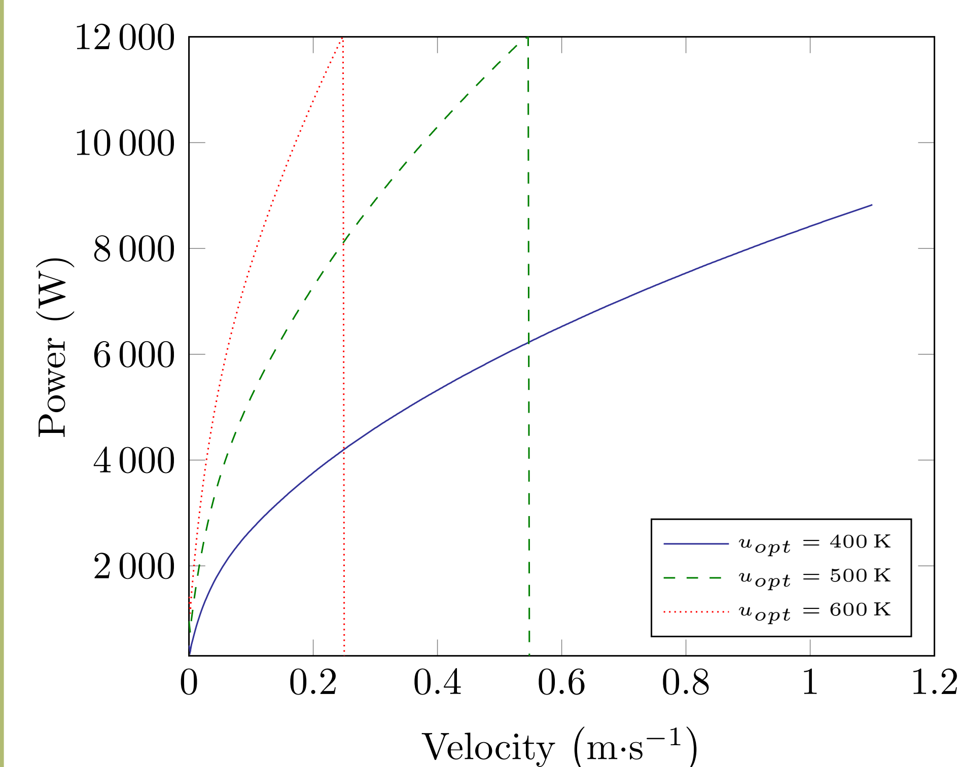
Process window when considering 8 plies
