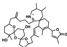
20-methyl spirolide G
