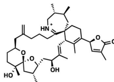
spirolide H
