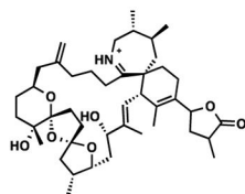
spirolide D
