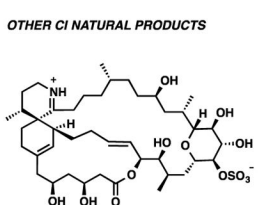
spiro-prorocentrimine
