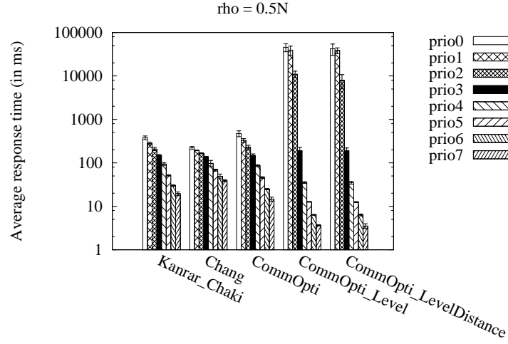
(b) High priority graph center positioning
