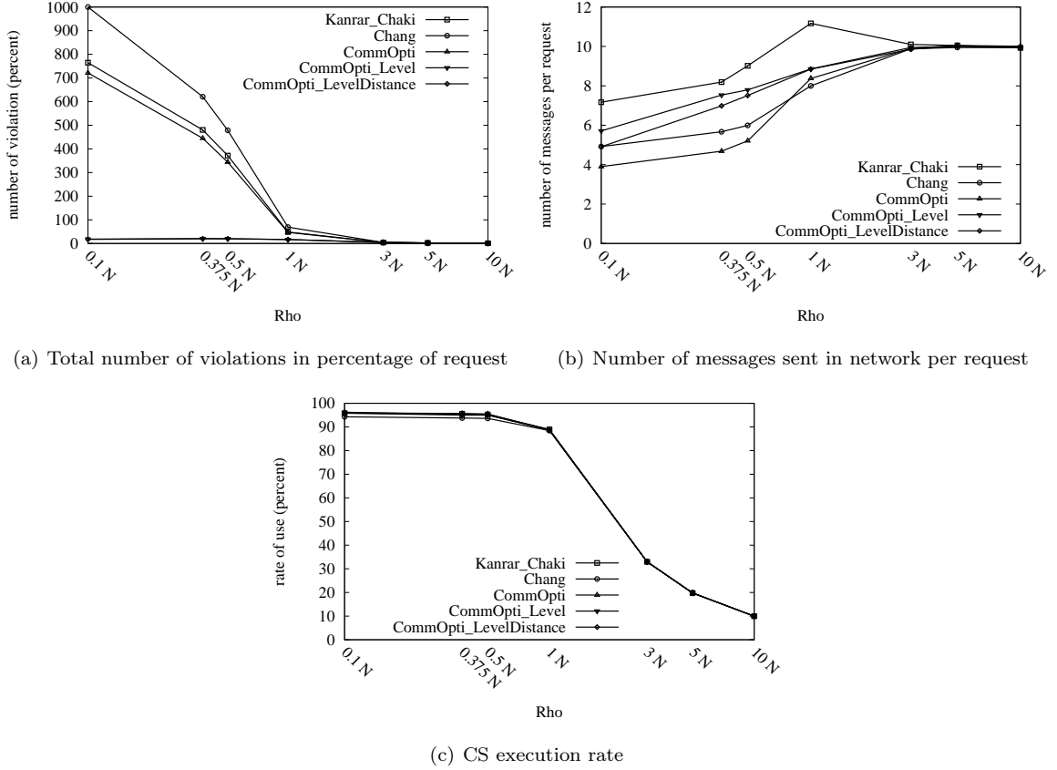
Figure 7: Impact of the load over the number of messages, CS execution rate, and the number of violations
