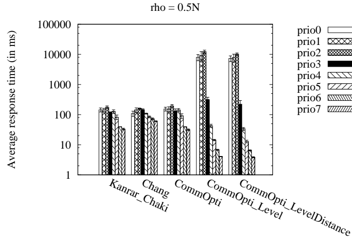
(c) Low priority graph center positioning
