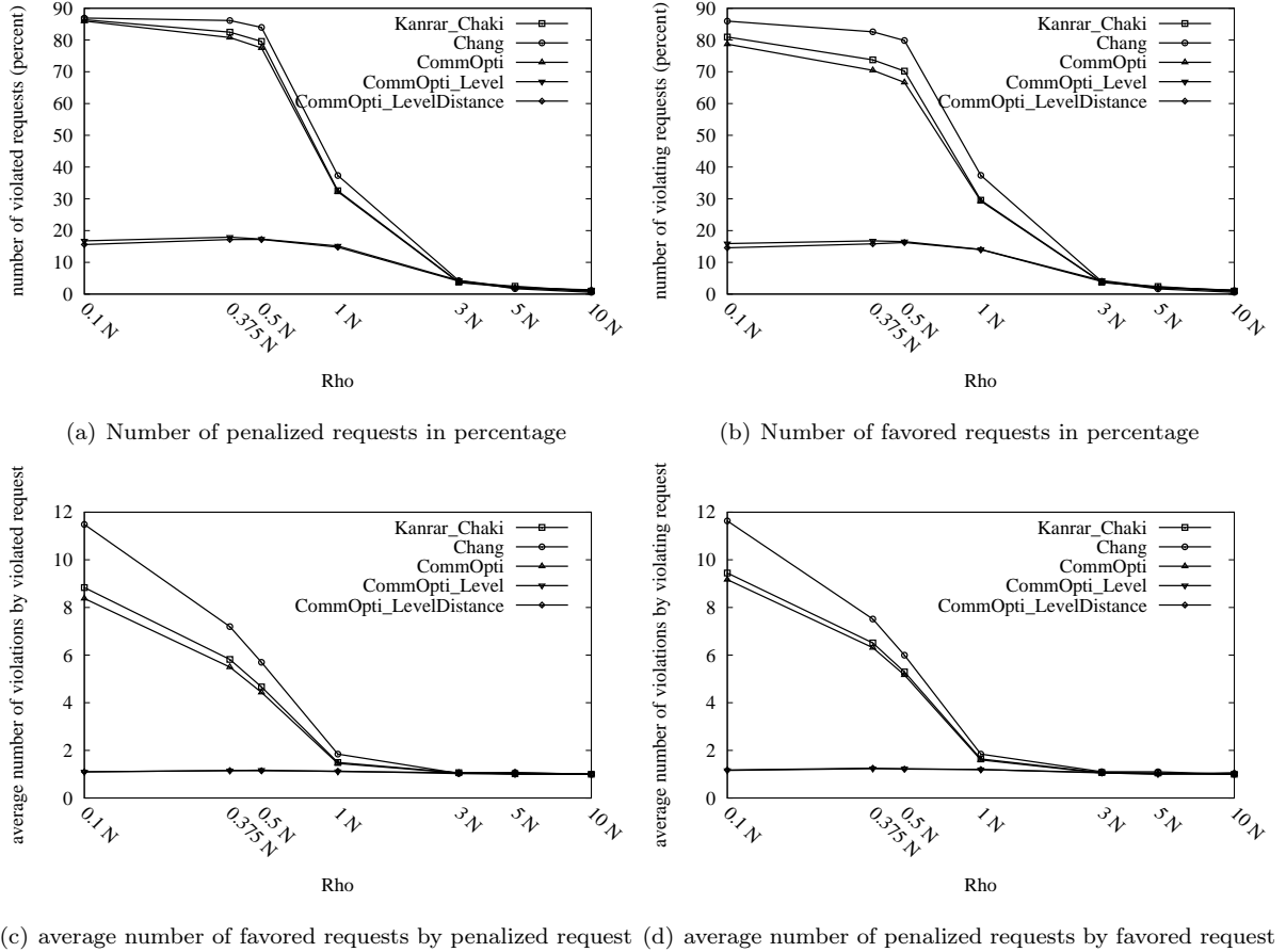
Figure 8: Impact of Load in Priority violation
