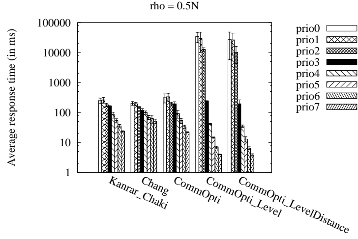
(a) Randomly priority positioning
