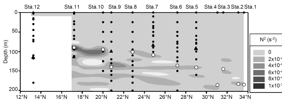
Figure 2. Vertical profiles of the Brunt-Väisälä buoyancy frequency ( N^2 ) calculated from the temperature–salinity measurements. The white circles display the thermocline depth and the black triangles display the depths of 1 % of photosynthetically active radiation (limit of the euphotic zone).
