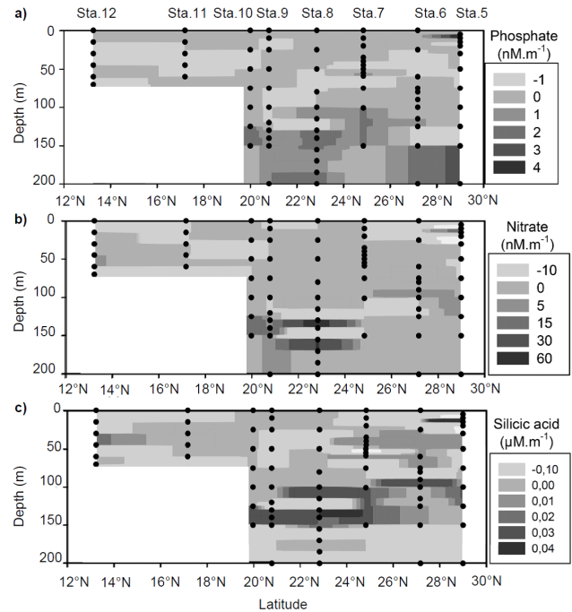
Figure 3. Vertical nutrient gradient ( d\text{Nutrient}/dz ) of Phosphate (a), Nitrate (b) and Silicic acid (c), between stations 5 and 12. The black dots display the sample depths and the names of the stations are indicated in the upper axes.
