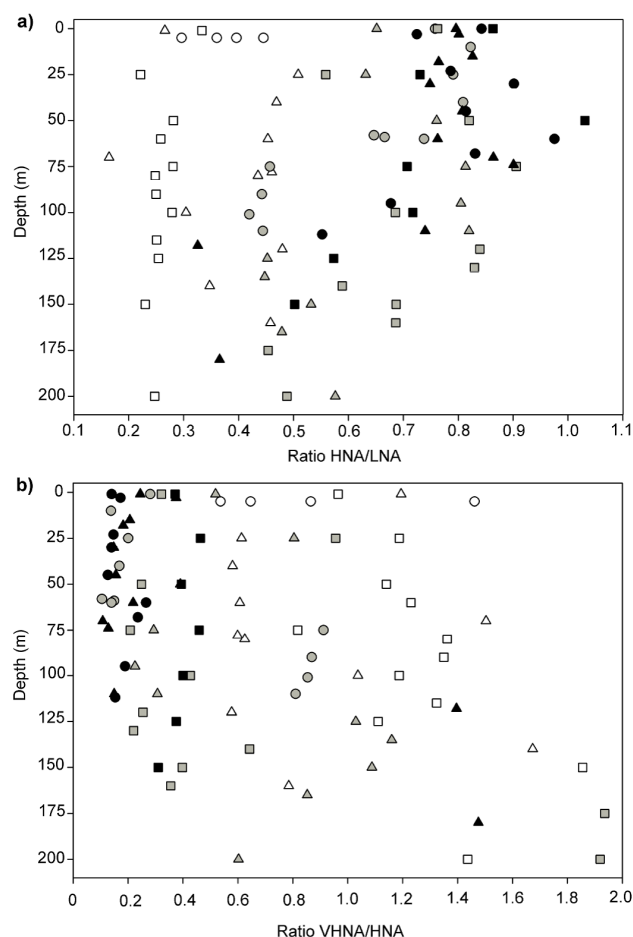
Figure 5. Ratios of the abundances between the heterotrophic prokaryote clusters according to depth. (a) shows the ratio of the abundances of HNA/LNA clusters while (b) shows the ratio of abundances of VHNA/HNA clusters. The white circles are stations 1, 2, 3, and 4. The white triangles and the squares are stations 5 and 6, respectively. The grey circles, triangles, and squares characterize stations 7, 8 and 9, respectively. The black squares, circles and triangles are stations 10, 11, and 12, respectively.
