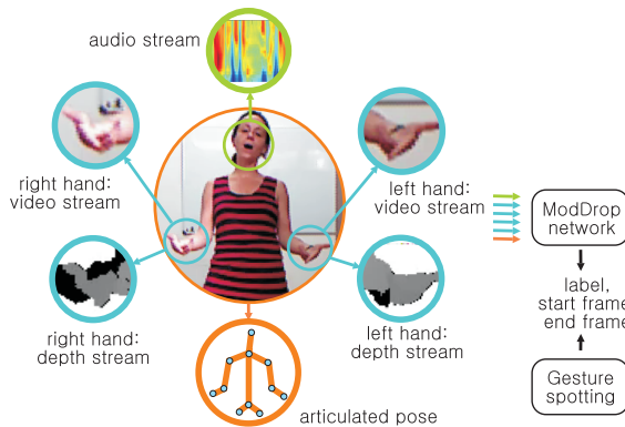
Fig. 1. Overview of our method on an example from the 2014 ChaLearn Looking at People (LAP) dataset.
