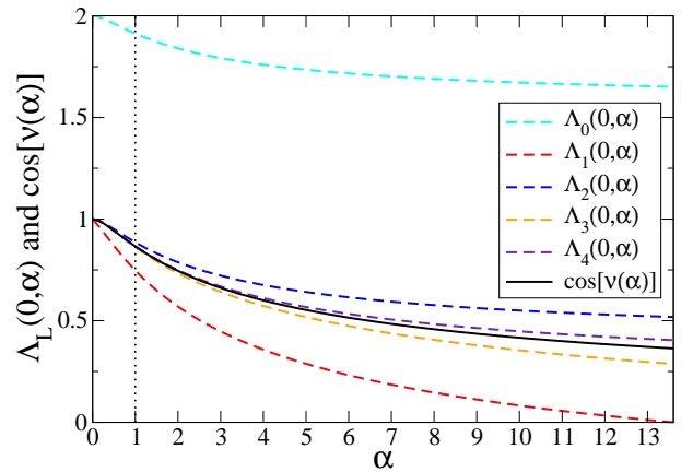
FIG. 2: (Color online) Analytically obtained borders of the continuous spectrum of M(s) ( s \in i\mathbb{R}^+ ) corresponding to the limits x \rightarrow \pm\infty . It is a collection of components characterized by an angular momentum quantum number L of a three-body asymptotic problem (not to be confused with the total angular momentum \ell of the four-body states), leading to a continuous set of eigenvalues ranging from \Lambda_L(0, \alpha) to \cos[\nu(\alpha)] for x \rightarrow -\infty , and ranging from \Lambda_L(0, 1/\alpha) to \cos[\nu(1/\alpha)] for x \rightarrow +\infty , where \alpha is the mass ratio given by Eq. (56), the \Lambda_L function is given by Eq. (78) and the mass angle \nu is given by Eq. (79). We plot \cos[\nu(\alpha)] (black solid line) and \Lambda_L(0, \alpha) (color dashed lines, with L = 0, 2, 4 from top to bottom above the solid line, and L = 1, 3 from bottom to top below the solid line) as functions of \alpha \in [0, \alpha_c(2; 1)] where \alpha_c(2; 1) is the critical mass ratio (83) for the Efimov effect in the \uparrow\uparrow\downarrow three-body problem. Due to the \alpha \leftrightarrow 1/\alpha symmetry of the 2+2 fermionic problem, one can restrict to \alpha \geq 1 (that is to the right of the vertical dotted line); the borders of the x \rightarrow -\infty continuum can then be directly read on the figure, and the ones of the x \rightarrow +\infty continuum can be obtained by mentally folding back the \alpha \leq 1 part of the figure into the \alpha \geq 1 part.
