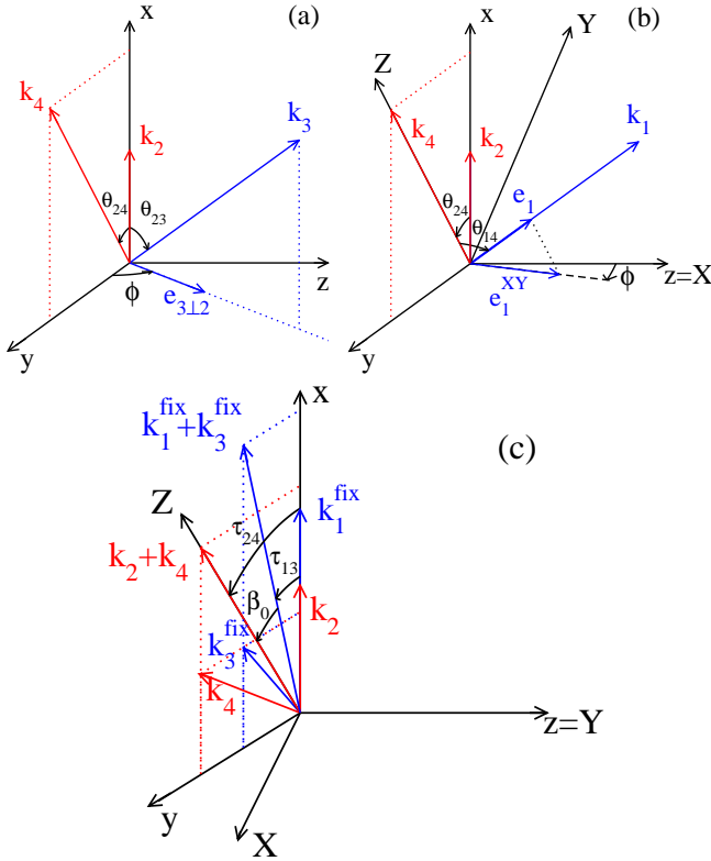
FIG. 1: (Color online) Positions and parametrisations of the wavevectors appearing in the angular integration in the functionals \mathcal{E}_{24,ij} . The vectors \mathbf{k}_2 and \mathbf{k}_4 are given by Eqs. (30,31). (a) For (i, j) = (2, 3) , \mathbf{k}_1 = -(\mathbf{k}_2 + \mathbf{k}_3 + \mathbf{k}_4) and one integrates over \mathbf{k}_3 using spherical coordinates of polar axis x and azimuthal axis y . (b) For (i, j) = (1, 4) , \mathbf{k}_3 = -(\mathbf{k}_1 + \mathbf{k}_2 + \mathbf{k}_4) and one integrates over \mathbf{k}_1 using the polar axis Z (direction of \mathbf{k}_4 ) and the azimuthal axis X (direction of \mathbf{e}_z ) as defined by Eq. (38), leading to the polar angle \theta_{14} and the azimuthal angle \phi ( < 0 in the figure). The dashed line gives the direction of the component \mathbf{e}_1^{XY} of \mathbf{e}_1 = \mathbf{k}_1/k_1 in the XY plane. (c) For (i, j) = (1, 3) , one integrates over the rotation \mathcal{R} , such that \mathbf{k}_1 and \mathbf{k}_3 are given by the action of \mathcal{R} on vectors \mathbf{k}_1^{\text{fix}} and \mathbf{k}_3^{\text{fix}} in the xy plane as in Eqs. (43,44), using the parametrisation in terms of Euler angles associated to the convenient axes X , Y and Z of Eq. (48).
