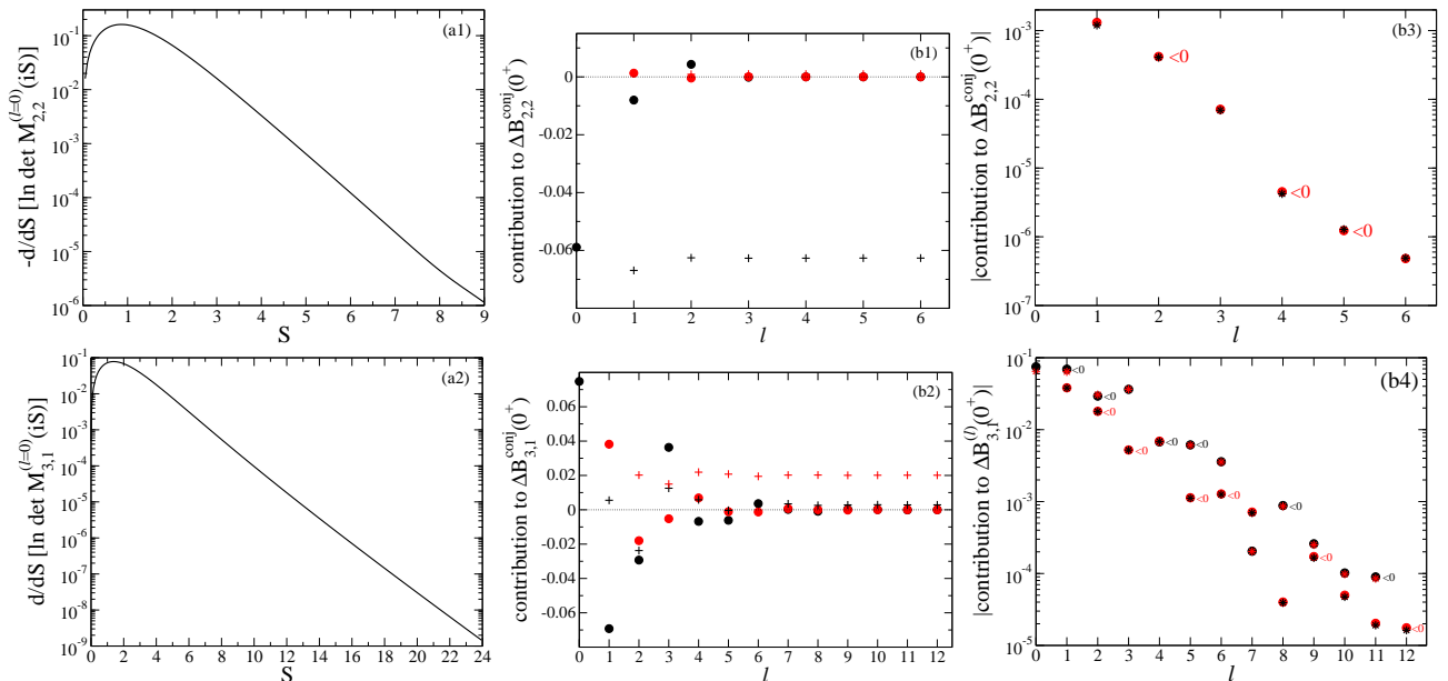
FIG. 7: Convergence in the integration over S and summation over \ell in Eq. (B10) (we recall that the mass ratio is \alpha = 1 ). (a) The logarithmic derivative of the determinant of M^{(\ell)}(iS) is a rapidly decreasing function of S ; the figure takes as an example (a1) the \ell = 0 channel of the 2 + 2 fermionic problem (for a numerical cut-off t_{\min} = -9 , thus without extrapolation; note the minus sign in the vertical axis), (a2) the \ell = 0 channel of the 3 + 1 fermionic problem. (b) The sum over \ell also seems to converge well, see the contribution of each angular momentum channel to the result (B10) for (b1) the 2 + 2 problem and (b2) the 3 + 1 problem: black disks for the parity sector (-1)^\ell , red disks for the parity sector (-1)^{\ell+1} ; the plus signs indicate the corresponding cumulative sums. Convincing evidence is even shown in (b3) for the 2 + 2 problem in the (-1)^{\ell+1} parity sector and in (b4) for the 3 + 1 problem in both parity sectors, where the numerical results (black disks for parity (-1)^\ell , red disks for parity (-1)^{\ell+1} ) are compared to the perturbative results (B53) and (B59) [red asterisks for parity (-1)^\ell , black asterisks for parity (-1)^{\ell+1} ] that extend to four bodies a technique developed for three bodies in reference [21] and are expected to be exact asymptotic equivalents for \ell \rightarrow +\infty (what is actually plotted is the absolute value of the results, so as to allow for a log scale, but their sign is indicated with the label “< 0” of the same color as the corresponding disks when they are negative: the negative black (red) disks are indicated with a black (red) “< 0” label; note that the black (red) asterisks have always the same sign as the corresponding red (black) disks).
