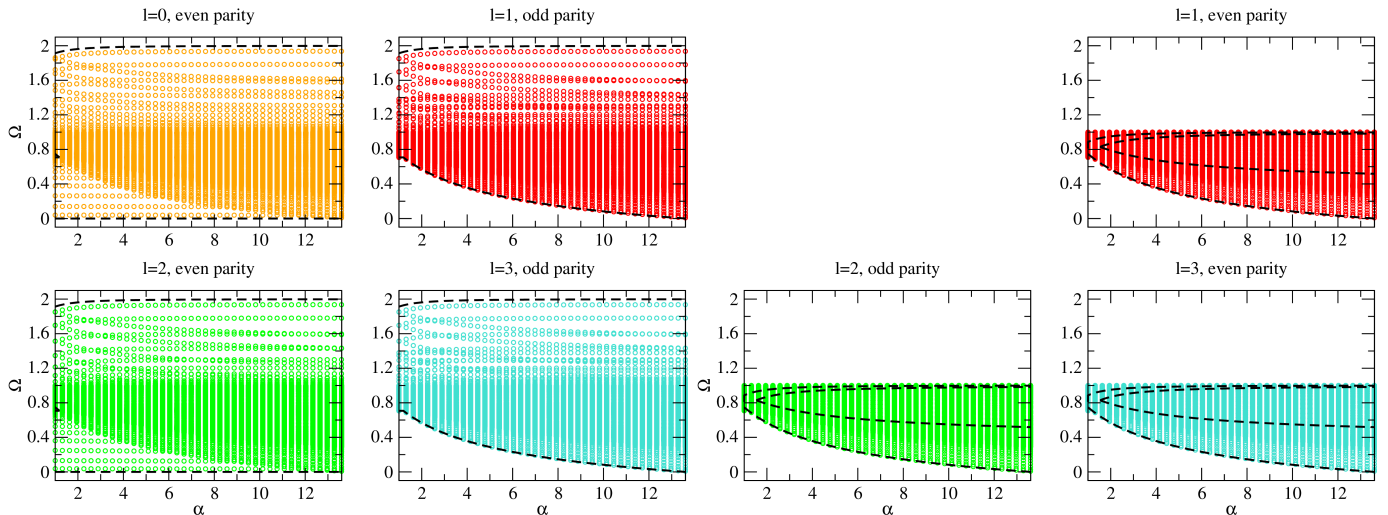
FIG. 3: Eigenvalues of M(s=0) as functions of the mass ratio \alpha \in [1, 13.6] , for various values of the angular momentum \ell and the parity, obtained numerically after discretisation and truncation of the variables x and \theta in the zone \rho \equiv [x^2 + (\pi - \theta)^2]^{1/2} > \rho_0 and of their log-polar versions t \equiv \ln(\rho/\rho_0) and \psi in the zone \rho < \rho_0 (see text): x_{\max} = -x_{\min} = 12 , dx = 1/5 , d\theta \simeq \pi/15 , \rho_0 = 2/5 , t_{\min} = -12 , dt = 1/5 , d\psi = \pi/15 , with the Gauss-Legendre integration scheme for the integrals over \theta and \psi , and the mid-point integration formula for the integrals over x and t . For the (-1)^{\ell+1} parity channels the \rho < \rho_0 zone is not useful and is not included in the numerics. The boundaries of the continuous spectrum of M(s) are given by black thick dashed curves: for the (-1)^{\ell+1} parity channels, this corresponds to the x \rightarrow \pm \infty continua of Eqs. (77,81) with all L \geq 1 ; for the (-1)^\ell parity channels, this corresponds to the x \rightarrow \pm \infty continua of Eqs. (77,81) with all L \geq 0 and to the (x, \theta) \rightarrow (0, \pi) [that is t \rightarrow -\infty ] continuum of Eq. (84). Contrarily to the 3 + 1 case, no eigenvalue of M(s=0) is found to cross zero for \alpha < \alpha_c(2; 1) = 13.6069\dots : no four-body Efimov effect is found for the 2 + 2 fermionic problem.
