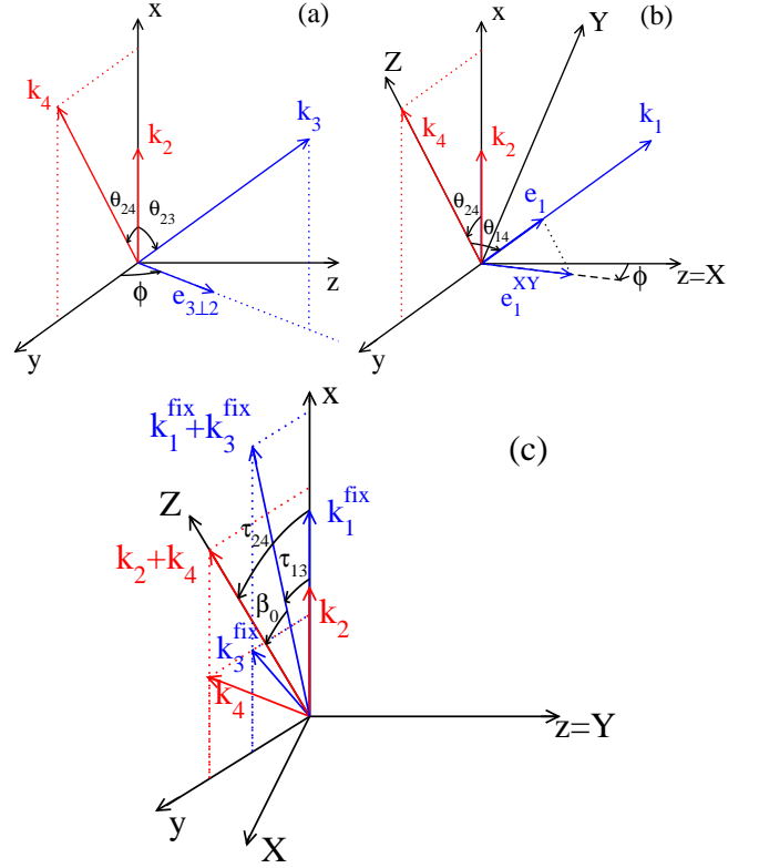
FIG. 1: (Color online) Positions and parametrizations of the wavevectors appearing in the angular integration in the functionals \mathcal{E}_{24,ij} . The vectors \mathbf{k}_2 and \mathbf{k}_4 are given by Eqs. (30,31). (a) For (i, j) = (2, 3) , \mathbf{k}_1 = -(\mathbf{k}_2 + \mathbf{k}_3 + \mathbf{k}_4) and one integrates over \mathbf{k}_3 using spherical coordinates of polar axis x and azimuthal axis y . (b) For (i, j) = (1, 4) , \mathbf{k}_3 = -(\mathbf{k}_1 + \mathbf{k}_2 + \mathbf{k}_4) and one integrates over \mathbf{k}_1 using the polar axis Z (direction of \mathbf{k}_4 ) and the azimuthal axis X (direction of \mathbf{e}_z ) as defined by Eq. (38), leading to the polar angle \theta_{14} and the azimuthal angle \phi ( < 0 in the figure). The dashed line gives the direction of the component \mathbf{e}_1^{XY} of \mathbf{e}_1 = \mathbf{k}_1/k_1 in the XY plane. (c) For (i, j) = (1, 3) , one integrates over the rotation \mathcal{R} , such that \mathbf{k}_1 and \mathbf{k}_3 are given by the action of \mathcal{R} on vectors \mathbf{k}_1^{\text{fix}} and \mathbf{k}_3^{\text{fix}} in the xy plane as in Eqs. (43,44), using the parametrisation in terms of Euler angles associated to the convenient axes X , Y and Z of Eq. (48).
