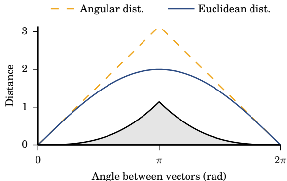
Figure 2.5: Impact of using Euclidean distance (solid blue line) instead of angle (dashed yellow line) between surface normal vectors. The shaded gray area represents the error.
