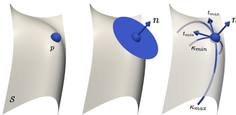
Figure 2.4: Representations (in dark blue) of a complex shape \mathcal{S} (in light gray) approximated as a 2D manifold. Left: no derivative (point). Middle: first derivative (plane). Right: second derivative (quadric).
