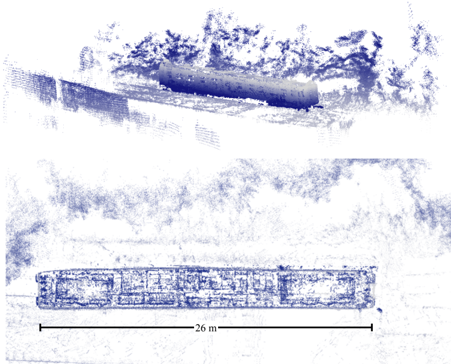
Figure 3.3: Deployment of the NiftiBot in a rail yard with a single railcar and dense vegetation. Top: Side view of the reconstructed environment with the railcar in the middle and the vegetation behind. Bottom: Top view of the reconstructed environment. For both images, colors of the point clouds were chosen to ease the comprehension of the 3D-scene.
