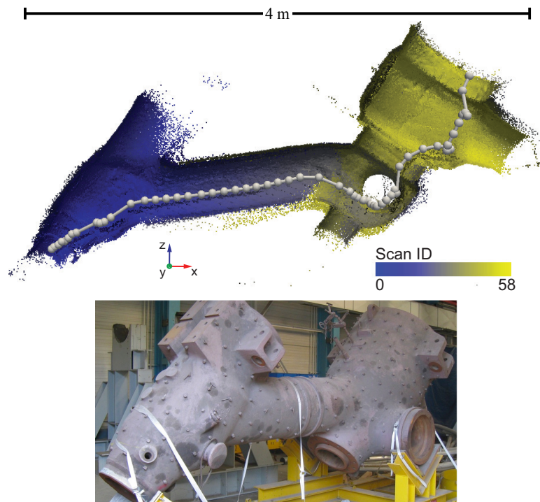
Figure 3.12: Deployment results of Magnebike in a real steam chest. Top: Cut view of the reconstructed environment. The light gray line correspond to the path of the robot, with the sphere being the positions where the robot stopped to take a 3D scan. The colors of the map follow the discrete time (from 0 to 58) at which the scans were taken. Bottom: The actual steam chest removed for maintenance.
