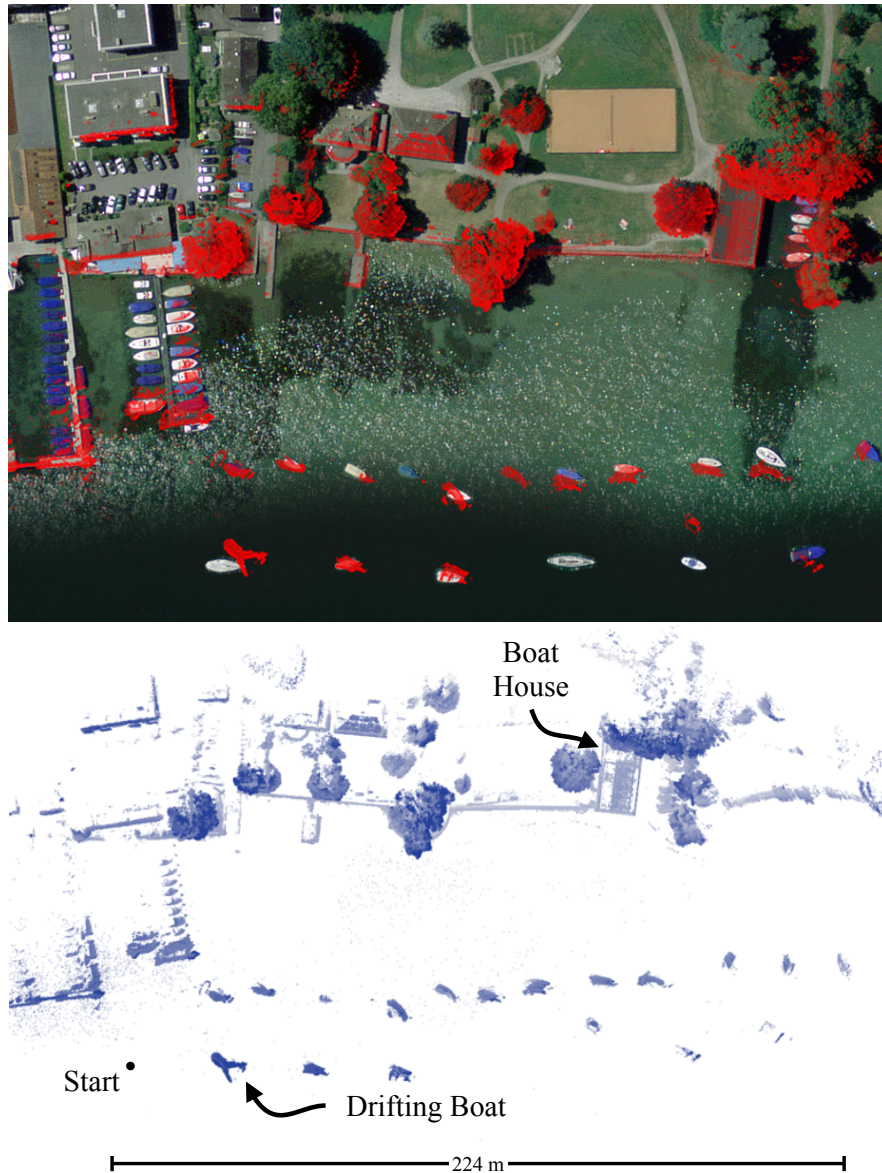
Figure 3.14: Reconstruction of the shoreline from a boat. Top: Overlay of the 3D map with an aerial view. Bottom: Top view of the 3D map with point colors based on elevation, light gray being low and dark blue being high. The orthogonal projection of the aerial image was provided by the Bundesamt für Landestopografie swisstopo (Art. 30 GeoIV): 5704 000 000
