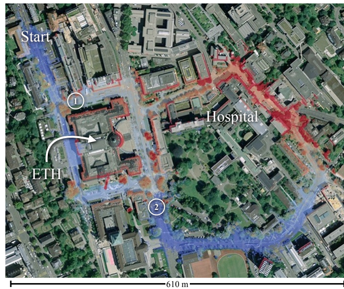
Figure 3.16: Overlay of a large scale reconstruction of the ETH main building and its surroundings with an aerial view. Colors represent the elevation, dark blue being low and dark red being high. Loop closing points are marked by numbers in circle, (1) being the small loop, (2) being the larger loop. The orthogonal projection of the aerial image was provided by the Bundesamt für Landestopografie swisstopo (Art. 30 GeoIV): 5704 000 000
