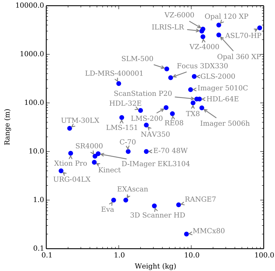
Figure 2.1: Classification of range sensors based on maximum range (m) and weight (kg). Manufacturers: Mesa Imaging (SR4000), ASUS (Xtion Pro), Microsoft (Kinect), Ocular Robotics (RE08), Hokuyo (URG-04LX, UTM-30LX), Sick (LMS-151, LMS-200, NAV350, LD-MRS-400001), Velodyne (HDL-64E, HDL-32E), FARO (Focus 3DX 330), Leica (ScanStation P20, ASL70-HP), RiegI (VZ-4000, VZ-6000), Topcon (GLS-2000), Trimble (TX8), Optec (ILRIS-LR), Zoller+Freohlich (Imager 5006h, Imager 5010C), KONICA MINOLTA (RANGE7), Panasonic (D-IMager EKL3104), Nikon (MMCx80), Artec (Eva), NextEngine (3D Scanner HD), Creaform (EXAscan), Renishaw (SLM-500), Fotonic (E-70 48W, C-70), Neptec (Opal 360 XP, Opal 120 XP). Note log scale.
