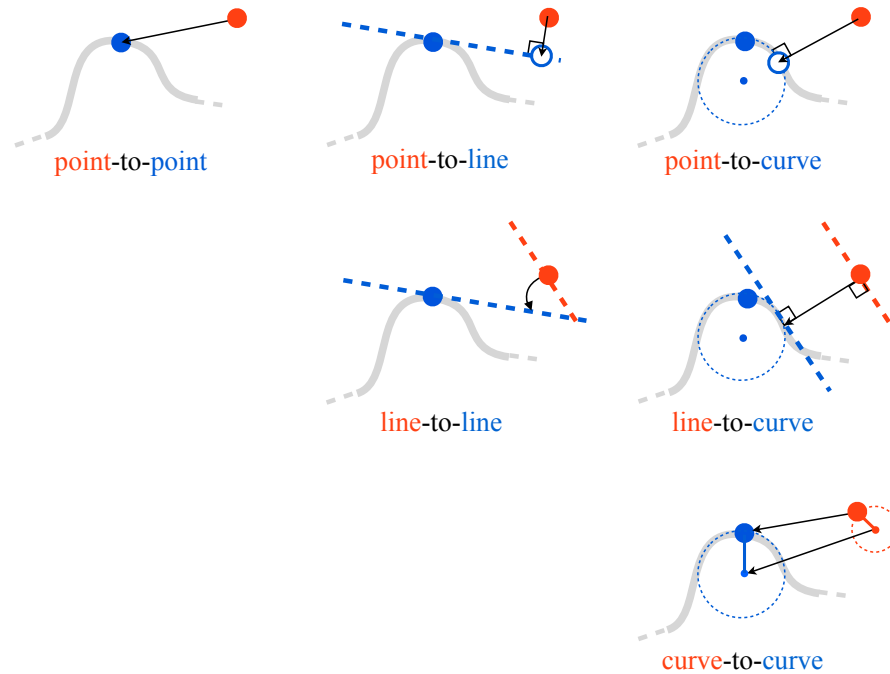
Figure 2.6: Possible morphing in 2D. The real underlying shape is represented in light gray with its approximation in dark blue. The misaligned surface is represented by a point in light red. The resulting errors are represented with black arrows.
