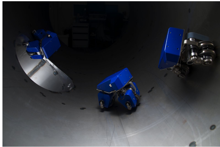
Figure 3.11: Three prototypes of chest inspection robots without the sensors, in a mock-up of a steam chest. The sensor was not installed at the time of the photograph.
