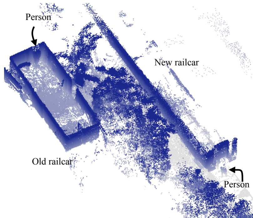
Figure 3.4: Bird's-eye view of the second experiment where the robot explored inside an old wooden railcar, crossed some dense vegetation and finished its path around a more modern railcar.
