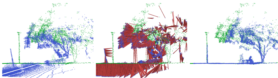
Figure 1.2: Examples of geometric registration between a reference point cloud (light green points) and a reading point cloud (dark blue points). Left: Initial position of the two point clouds. Middle: Alignment error (dark red lines). Right: Final alignment of the two point clouds.
