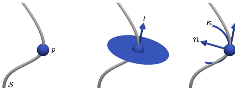
Figure 2.3: Representations (in dark blue) of a complex shape \mathcal{S} (in light gray) approximated as a 1D manifold. Left: no derivative (point). Middle: first derivative (line). Right: second derivative (curve).
