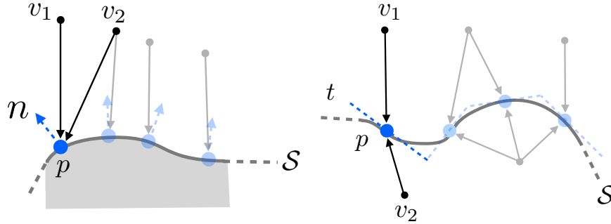
Figure 2.2: Difference between using normal vectors and tangent vectors to represent a 2D shape S . Left: The 2D line is known to be measured from a volume, which can only view from one side as illustrated with the black arrows \mathbf{v}_1 and \mathbf{v}_2 . The direction of the surface make sense to be encoded in its representation leading to the choice of normal vectors \mathbf{n} (dashed blue arrow). Right: The same line can be observe from both direction leading to the selection of an undirected tangent vector \mathbf{t} (dashed blue line).
