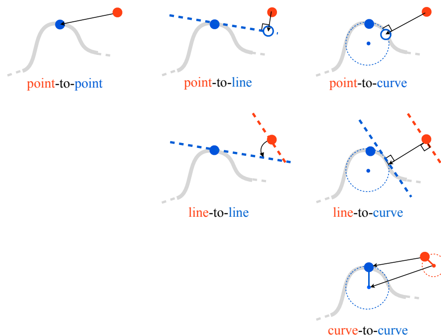
Figure 2.6: Possible morphing in 2D. The real underlying shape is represented in light gray with its approximation in dark blue. The misaligned surface is represented by a point in light red. The resulting errors are represented with black arrows.
