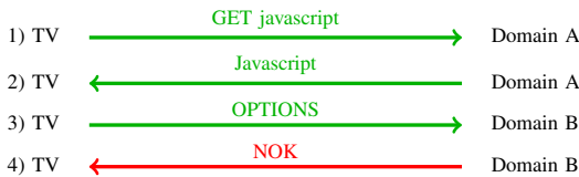
Fig. 5. Same-origin security compliant browser
