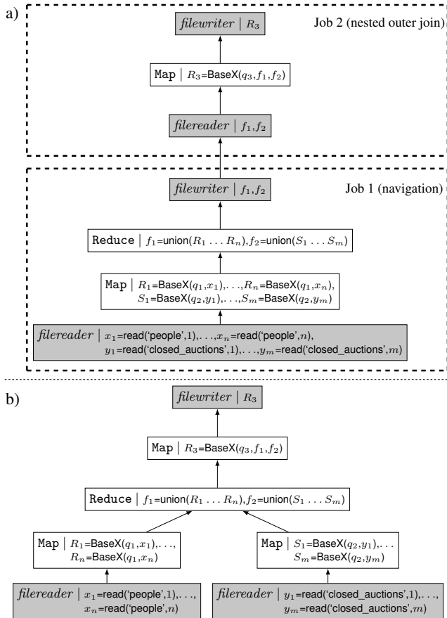
Figure 5: Execution of XQuery using alternative architectures based on MapReduce (a) and PACT (b) for comparison with PAXQuery.
