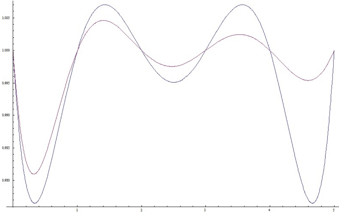
FIGURE 1 – The Arm function for k = 6 and k = 7
