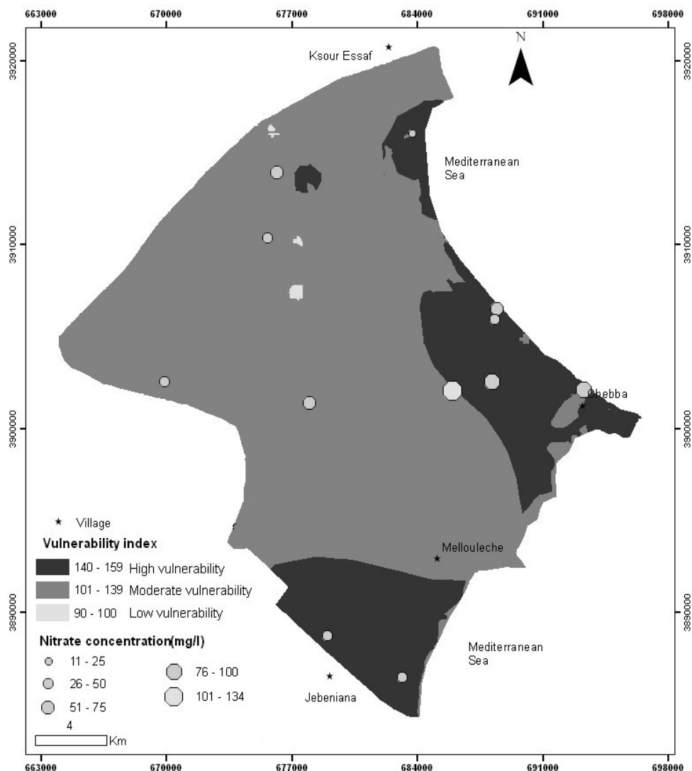
Fig. 3. Groundwater vulnerability and nitrate distribution in the Chebba - Mellouleche Aquifer using DRATIC method (Saidi, 2011).
