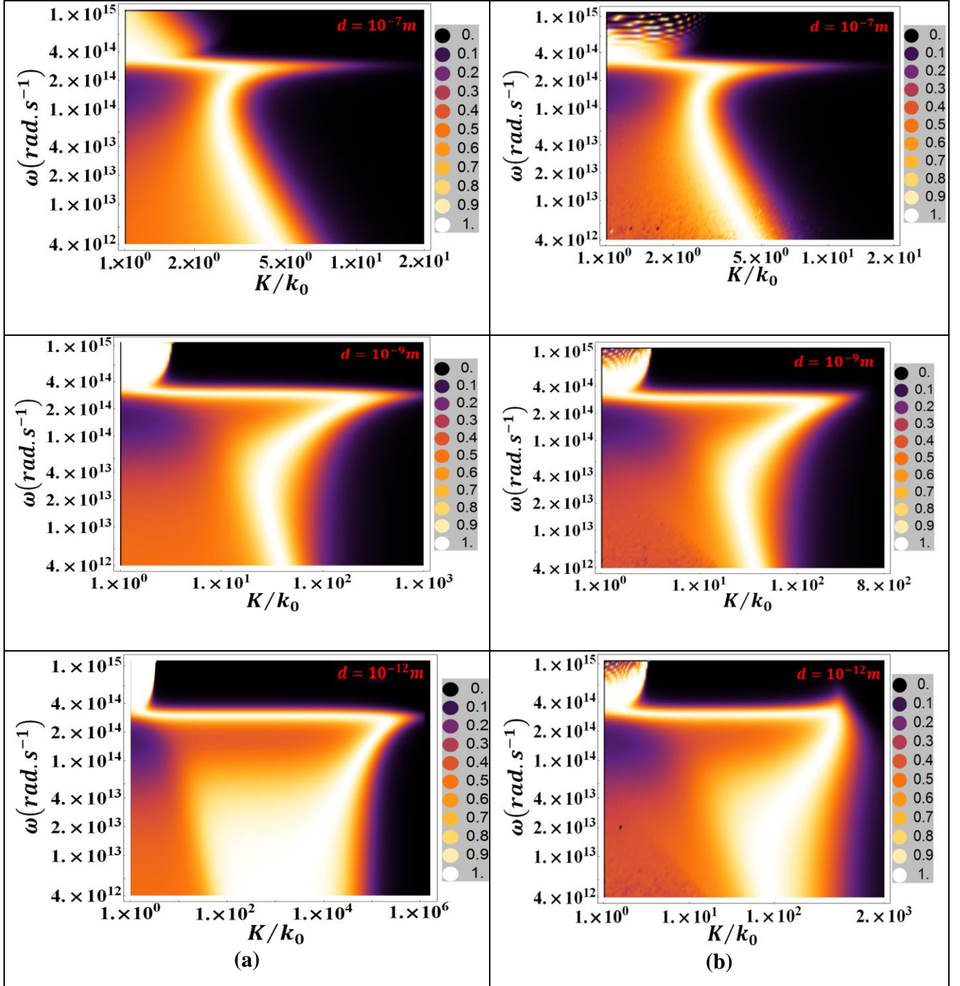
Figure 4: Plot of the transmission coefficient 4(Im(r_{31}^P))^2 e^{2i\gamma_3 d} / |1 - (r_{31}^P)^2 e^{2i\gamma_3 d}|^2 of the p -polarized evanescent EM waves in the plane (\omega, K) for the local model case (a) and the nonlocal model case (b) for the doping level N = 10^{20} \text{ cm}^{-3} and average temperature T = 300\text{K} and at different separation distances d .
