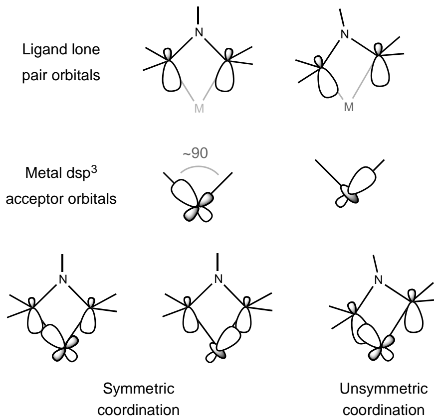
Figure 9. Orientation of the lone pair orbitals of in DPPA-type ligands (above), of the metal dsp^3 hybrids (center) and misalignment of the two types of orbitals (below).
