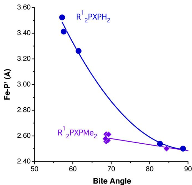
Figure 10. Dependence of the calculated long Fe-P' bond distance on the bite angle in the series of complexes [\text{FeCl}_2(\text{SMe}_2)(\text{R}^1_2\text{PXP H}_2)] (circles) and [\text{FeCl}_2(\text{SMe}_2)(\text{R}^1_2\text{PXP Me}_2)] (rhombuses), with X = NMe, C 2 H 4 , C 3 H 6 ; R 1 = H, Me, Ph.
