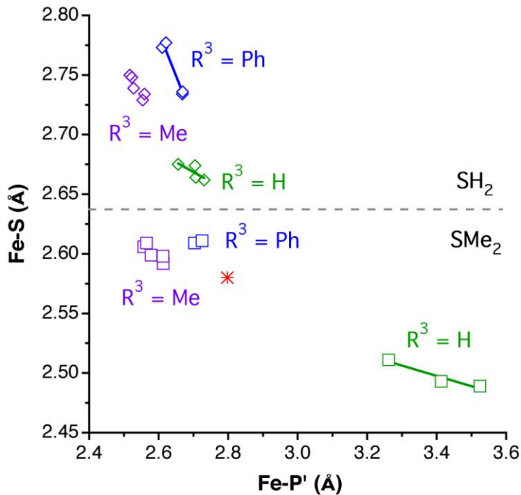
Figure 5. Scatterplot of the long Fe-P' vs. the Fe-S bond distances in the series of calculated complexes [\text{FeCl}_2(\text{SR}_2)\{\text{R}^1_2\text{PN}(\text{R}^2)\text{P}'\text{R}^3_2\}] ( \text{R} = \text{H}, \text{Me} ; \text{R}^1, \text{R}^2, \text{R}^3 = \text{H}, \text{Me}, \text{Ph} ). The asterisk indicates the experimental values for 3 .
