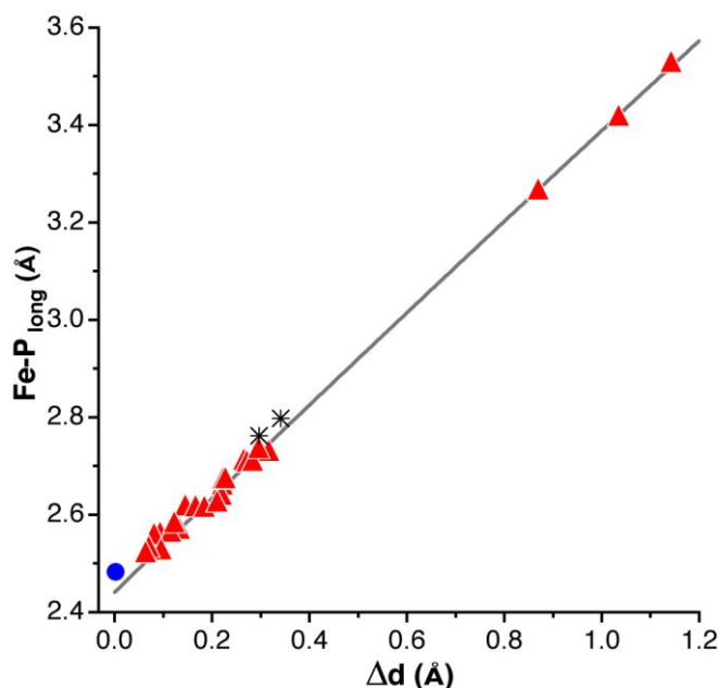
Figure 4. The long Fe-P' distance in the high spin complexes [\text{FeCl}_2(\text{SR}_2)\{\text{R}^1_2\text{PN}(\text{R}^2)\text{P}'\text{R}^3_2\}] (R = H, Me; R 1 , R 2 and R 3 = H, Me, Ph) plotted as a function of the degree of unsymmetry between the two Fe-P bond distances ( \Delta d ) in bidentate diphosphinoamines (triangles), optimized at the BP86 level, including a transition state for [\text{FeCl}_2(\text{SMe}_2)\{\text{Me}_2\text{PN}(\text{Me})\text{PMe}_2\}] (circle) and the corresponding values in the experimental structures 3 and 4 (asterisks). Geometric parameters are given in Table 2.
