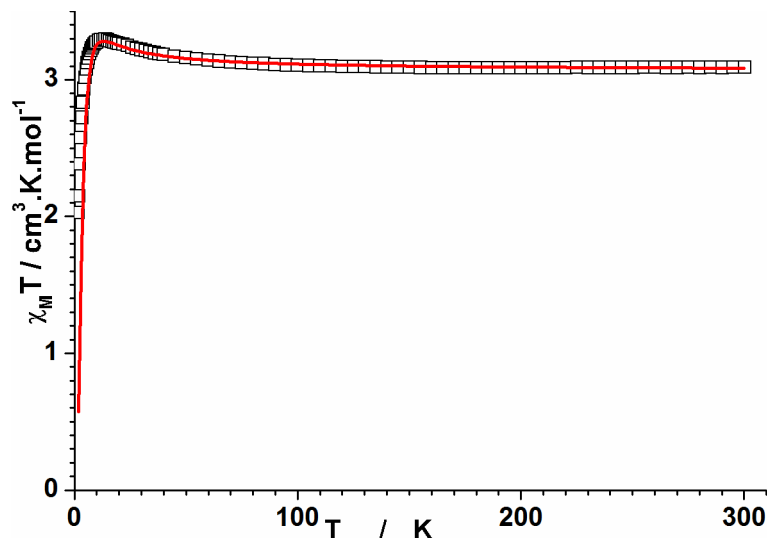
Figure 11. Evolution of the magnetic susceptibility \chi_M product with temperature for complex 3 , measured in a static 1 T field, the red line is the fit resulting from the parameters described in the text.
