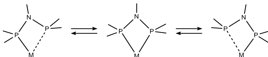
Figure 6. Interconversion between two unsymmetrically-coordinated phosphorus atoms of DPPA-type ligands.
