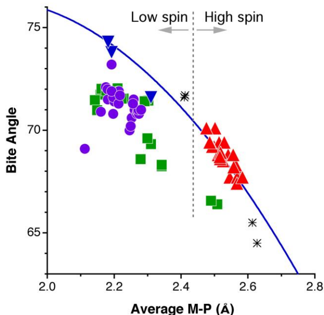
Figure 7. Scatterplot of the calculated average Fe-P bond distances and bite angles in the series of high (up-pointing triangles) and low spin (down-pointing triangles) Fe(II) complexes with SR_2 and R^1_2PN(R^2)PR^3_2 ligands (Table 2). Experimental data for related complexes of iron (circles) and other metals (squares) also shown for comparison. Compounds 3-6 are represented by asterisks and the continuous line corresponds to a least-squares fitting of the calculated values (three points with M-P > 2.8 \text{ \AA} not shown were included in the fitting).
