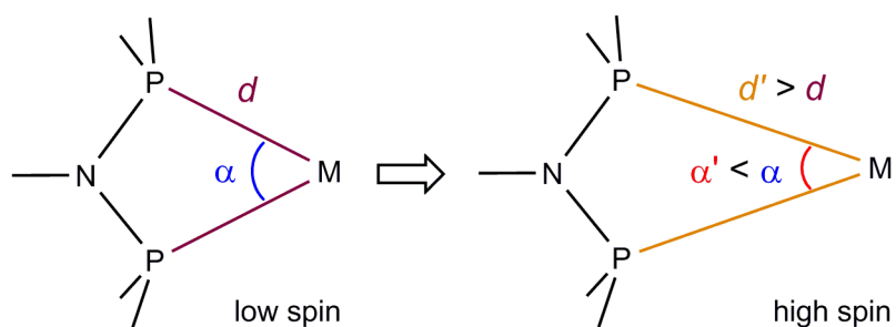
Figure 8. Geometrical differences in the chelate ring formed by PNP ligands between the low and high spin states of transition metal complexes: a high average M-P distance is associated with a smaller P-M-P angle and a larger P-N-P angle (see also Figure 7).
