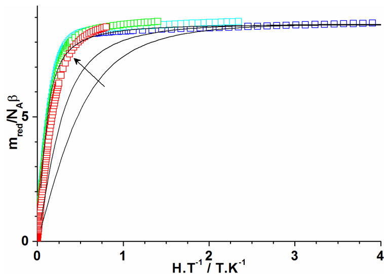
Figure 13. Plots of the reduced isothermal magnetization vs. field for complex 4 (1.8 (dark blue), 3 (light blue), 5 (green) and 8 (red) K). Black lines are the Brillouin curves corresponding successively to two S = 2 with g = 2.18 , one S = 4 with g = 2.18 , and 1/3 \times one S = 12 with g = 2.17 .
