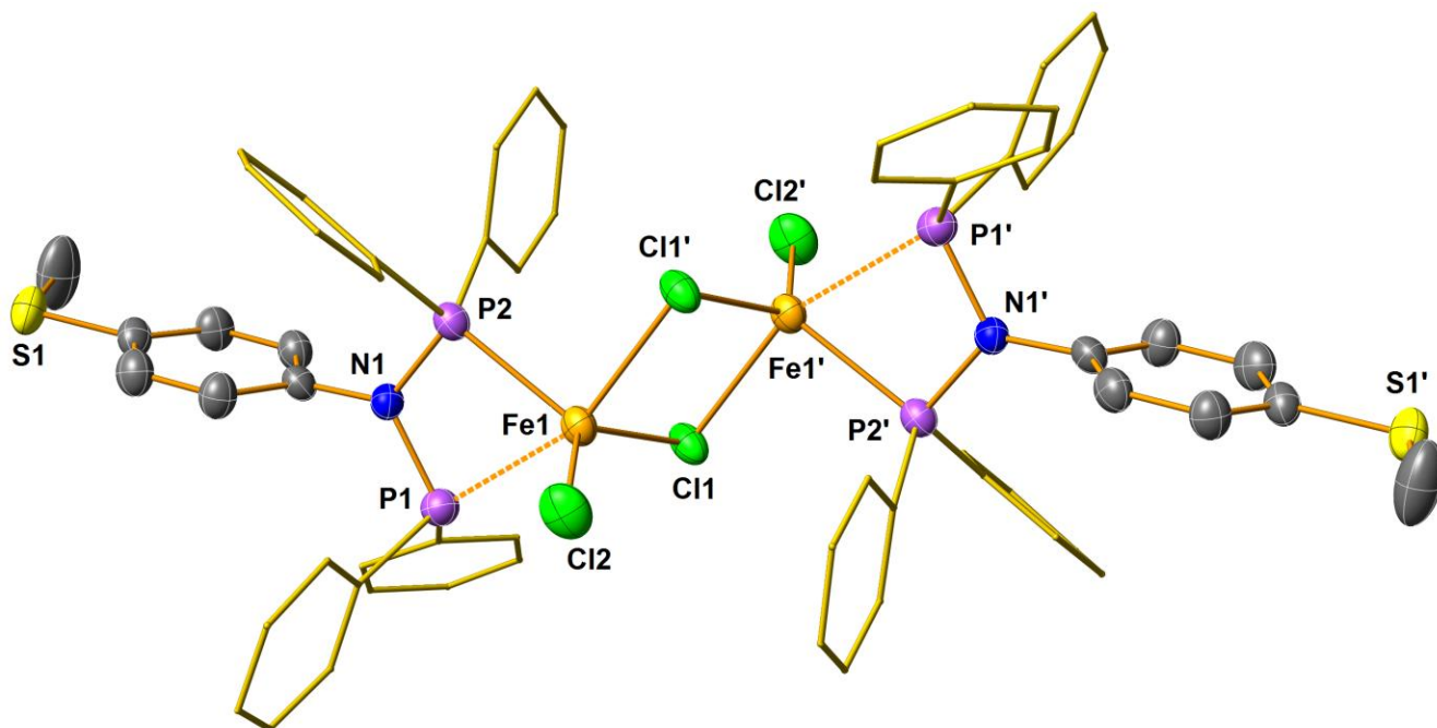
Figure 2. View of the molecular structure of 4 . Hydrogen atoms omitted and P-phenyl substituents represented in stick style for clarity. Ellipsoids are represented at 50% probability level. Selected bond distances and angles are summarized in Table 1.
