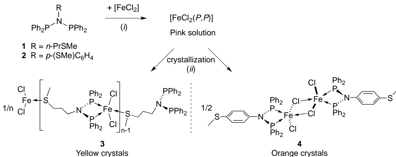
Scheme 1. Synthesis of the Fe(II) complexes 3 and 4 . Conditions: (i) \text{CH}_2\text{Cl}_2 , room temp., 12 h; (ii) reduction of the original reaction volume to 1/3 followed by layering with pentane.
