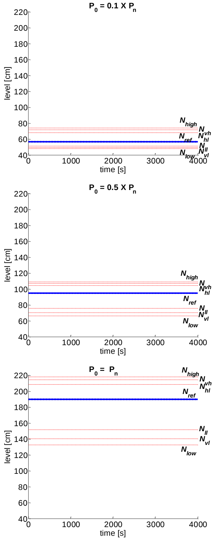
Fig. 2. Set point for N_{rl} at different power rate P_o values.
