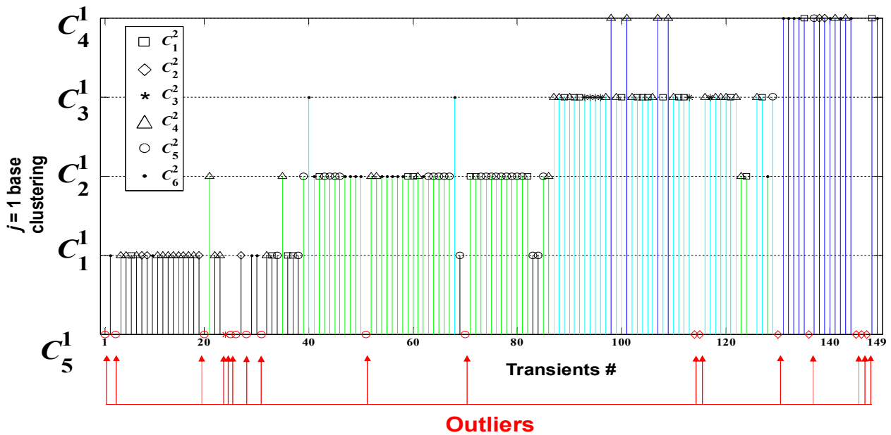
Figure 16: The 149 transients in chronological order along with the j=1 and j=2 base clustering results.
